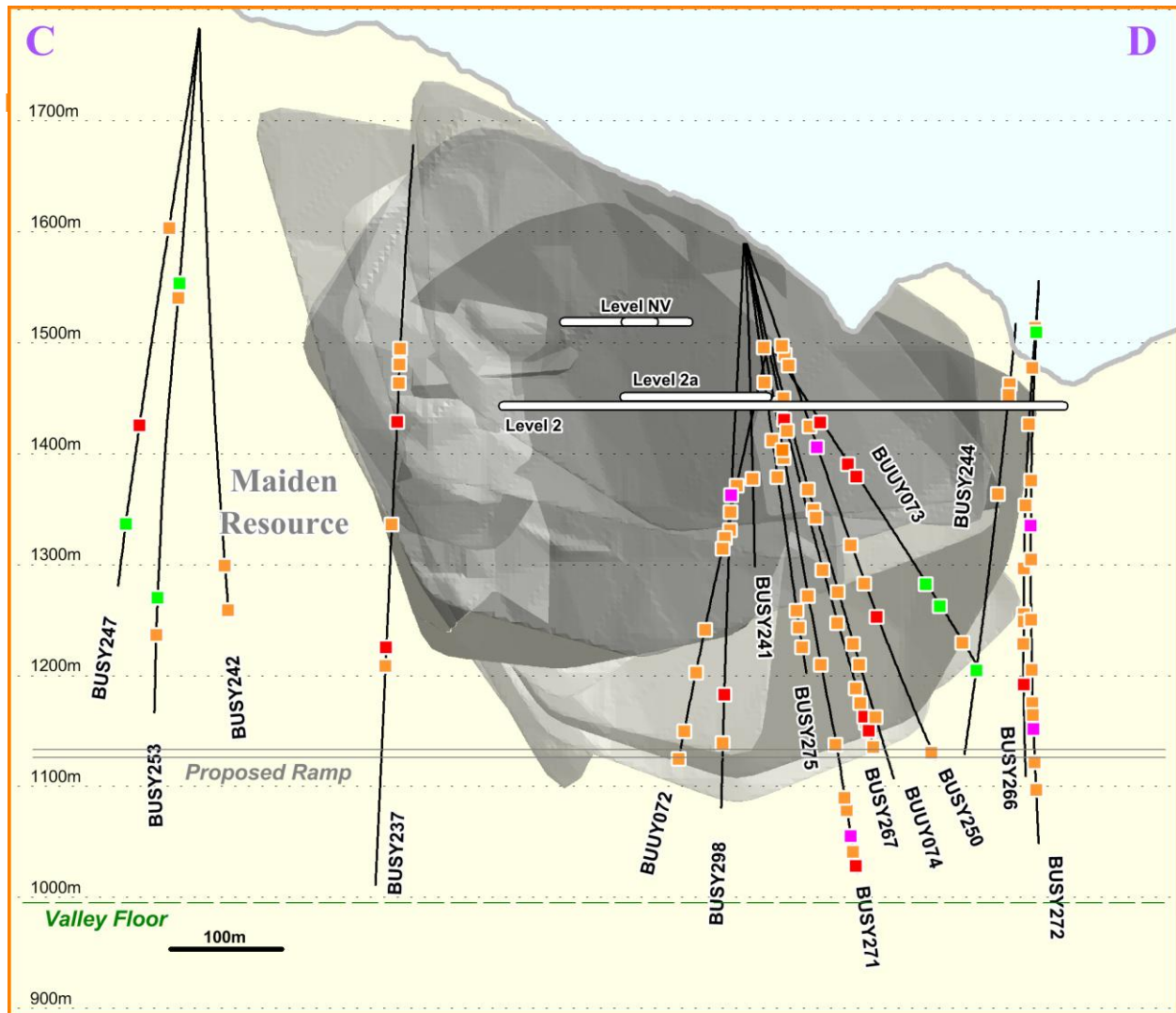
Figure 2 – Longitudinal Section of Yaraguá Drilling Highlights & Plan View of Underground Sampling
