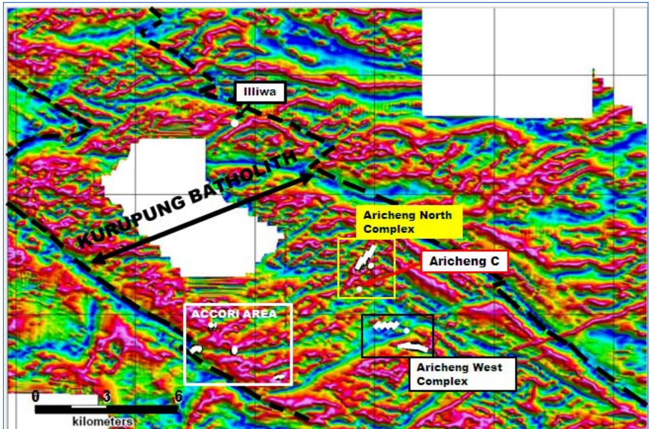
Figure 1 – Multiple Uranium-Bearing Structures in the Kurupung Batholith
