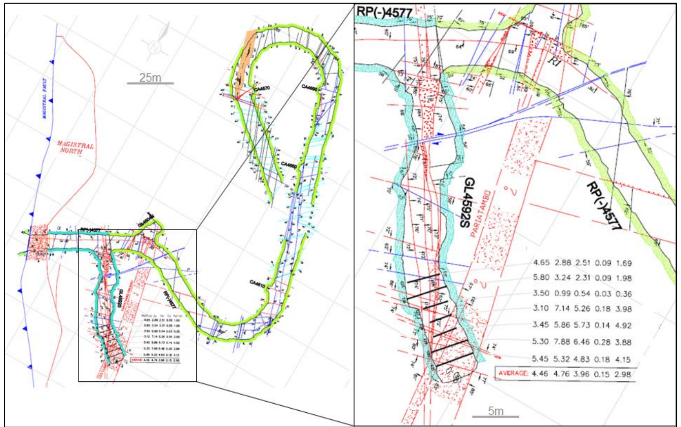
Figure 4: Underground plan illustrating Channel sample locations on new footwall mineralized zone at Magistral North Deposit
