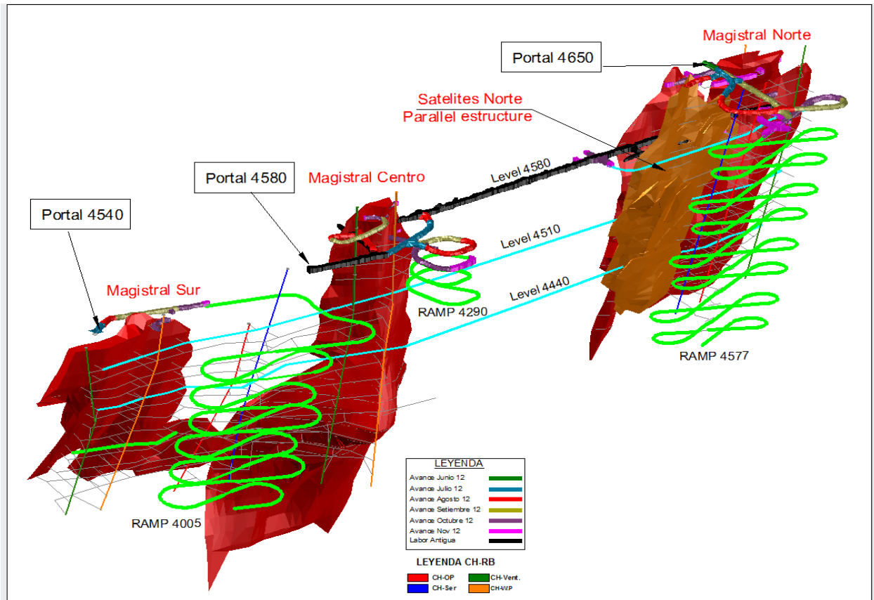
Figure 3: Underground development progress and plan on Magistral North, Central and South deposits at Santander Mine. Note presence of potentially significant satellite zone in the footwall to the Magistral North deposit.
