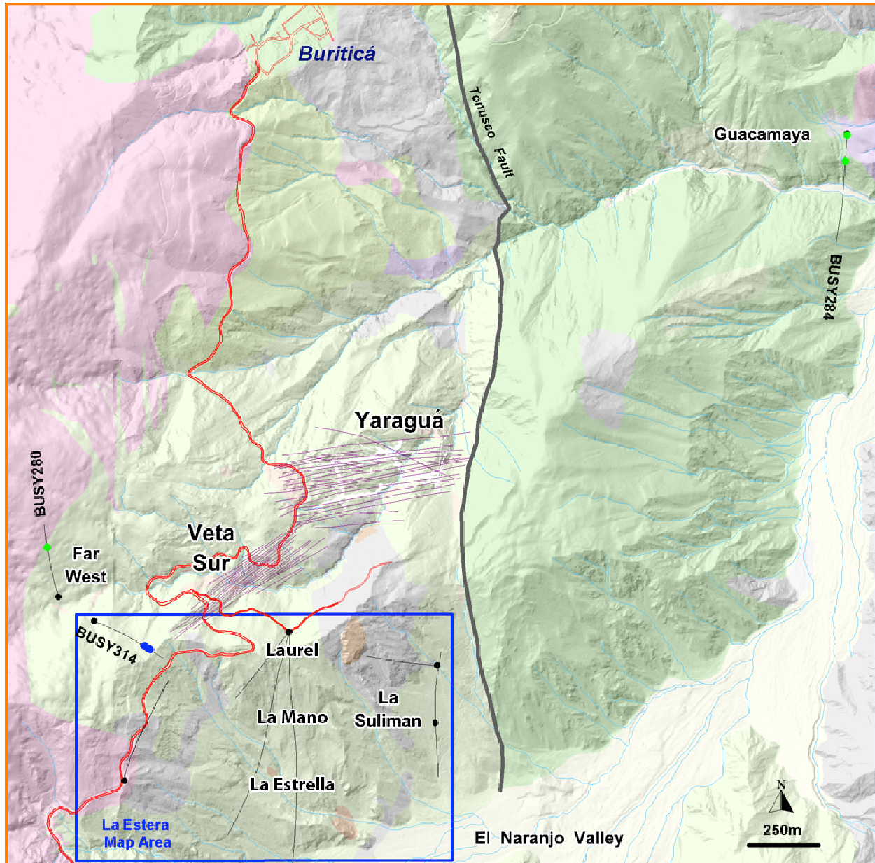
Figure 1 – Plan View of new drilling highlights, showing the surface projection of veins in the October 2012 mineral resource model on geology-topography base.
