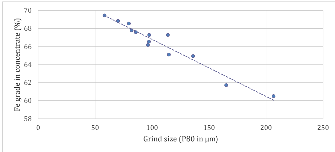
Figure 1: Product grade versus grind size (P80)
