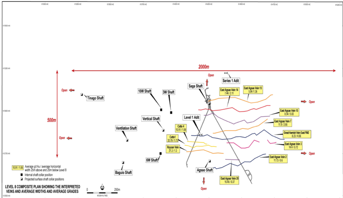
Figure 1. Level 8 plan showing planned development and veins with average grades and widths. The veins are open in all directions.
