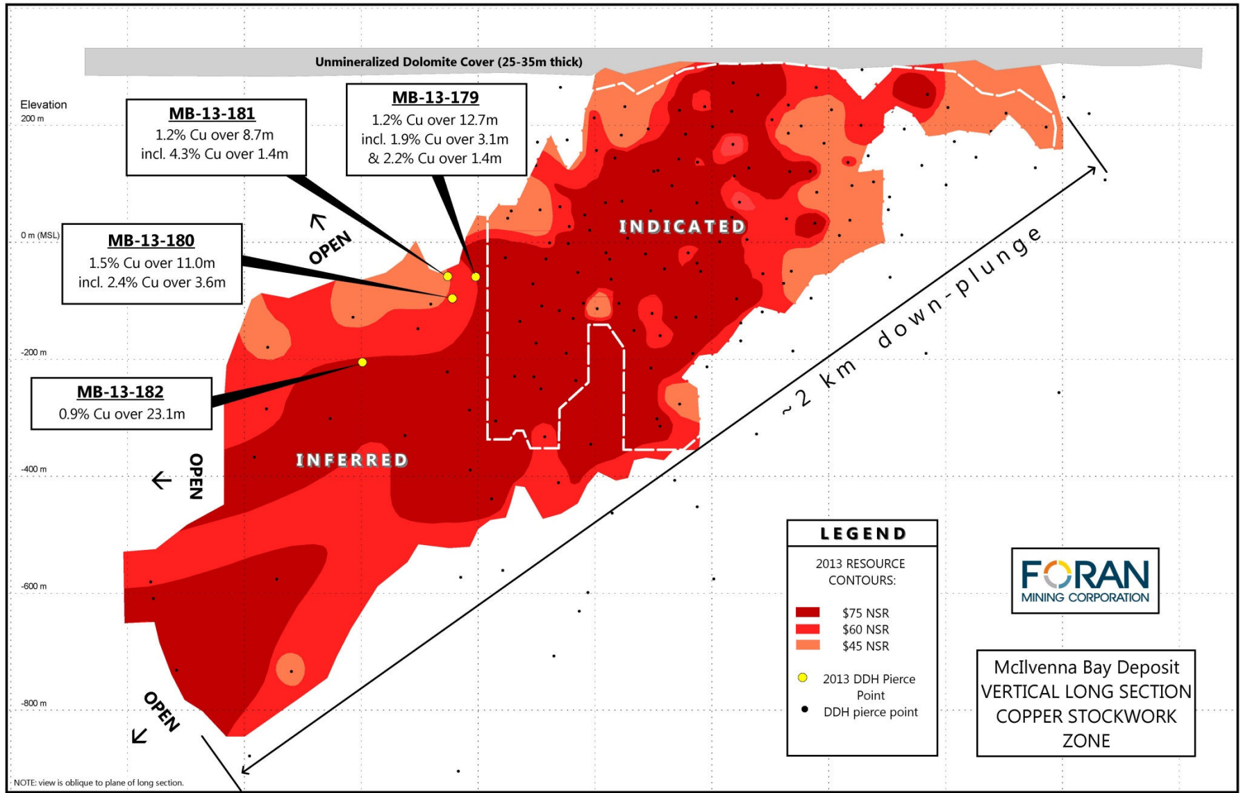
Figure 1. McIlvenna Bay Deposit Copper Stockwork Zone Longitudinal Section with diamond drill hole pierce points.
