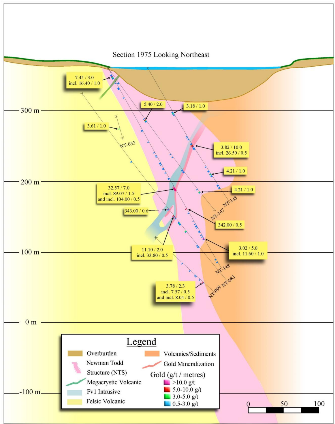
Figure 2: Cross Section 1975NW Illustrating Possible Lithological Control on Higher-Grade Mineralization
