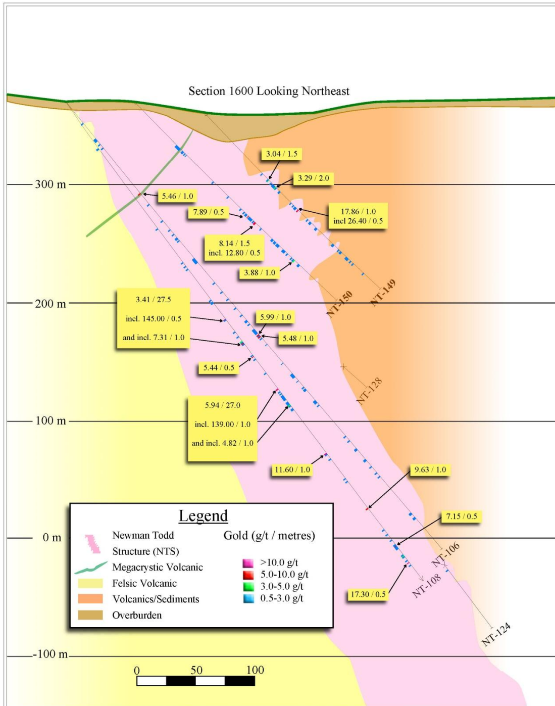
Figure 1: Cross Section 1600NW Showing Geology and Assay Highlights
