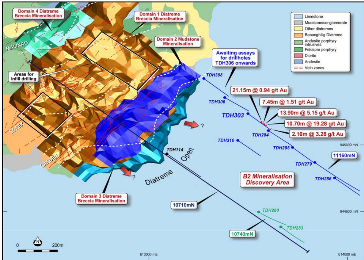
Figure 1. Bananghilig geology map showing the B2 drill hole locations.
