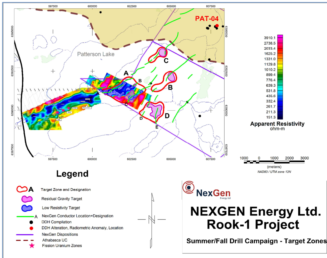
Fig 1 Rook I Project – Principal Target Areas
