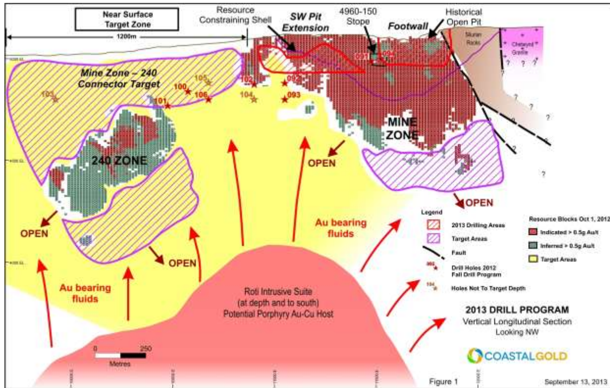
FIGURE 1: 2013 RESOURCE DRILL PROGRAM VERTICAL LONGITUDINAL SECTION
