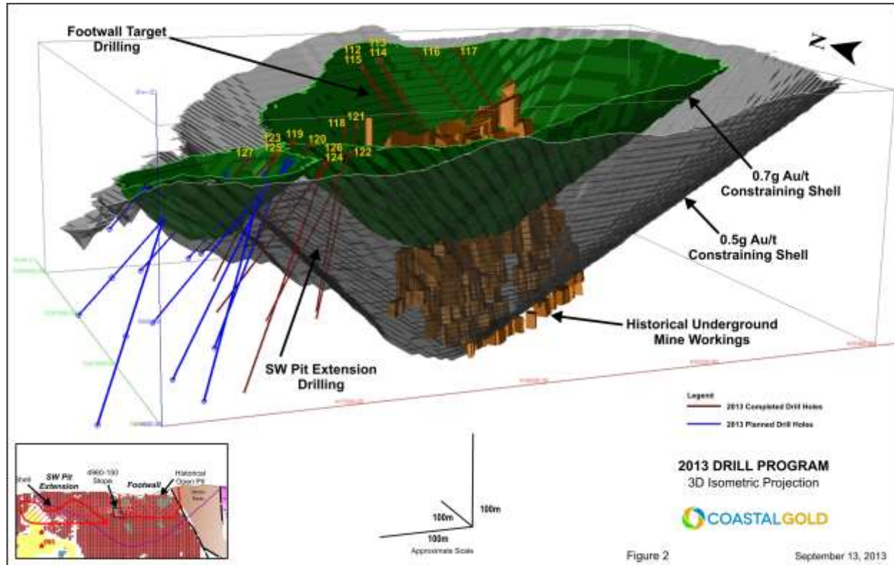
FIGURE 2: 2013 RESOURCE DRILL PROGRAM 3D ISOMETRIC PROJECTION
