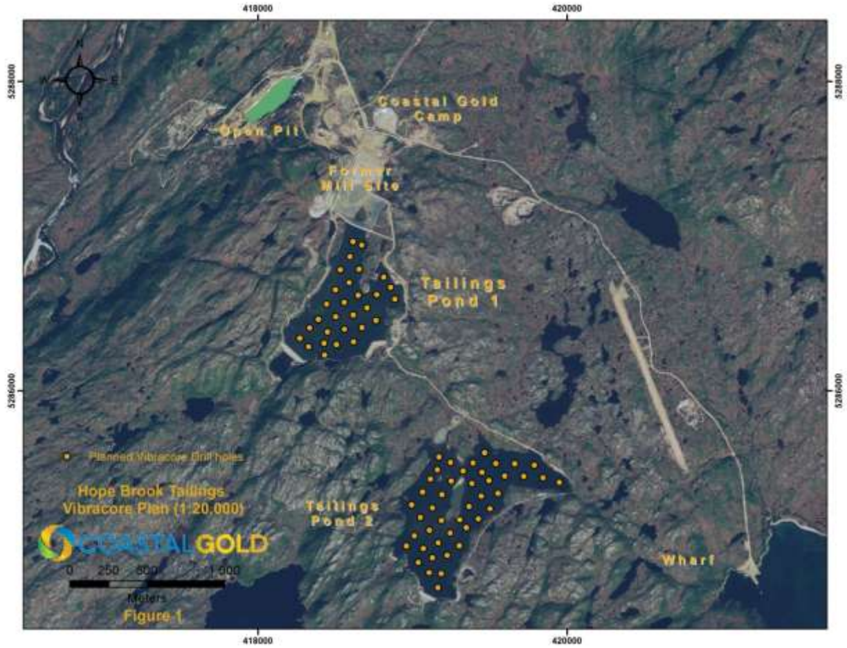
FIGURE 1: VIBRACORE TAILINGS DRILL PROGRAM, HOPE BROOK GOLD PROJECT
