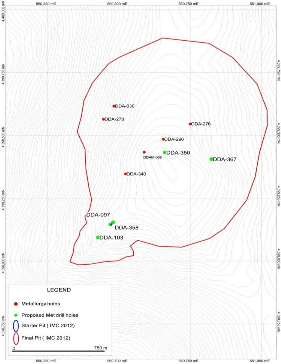
Figure 1: Erato Metallurgical Sample Drill Hole Location Map
