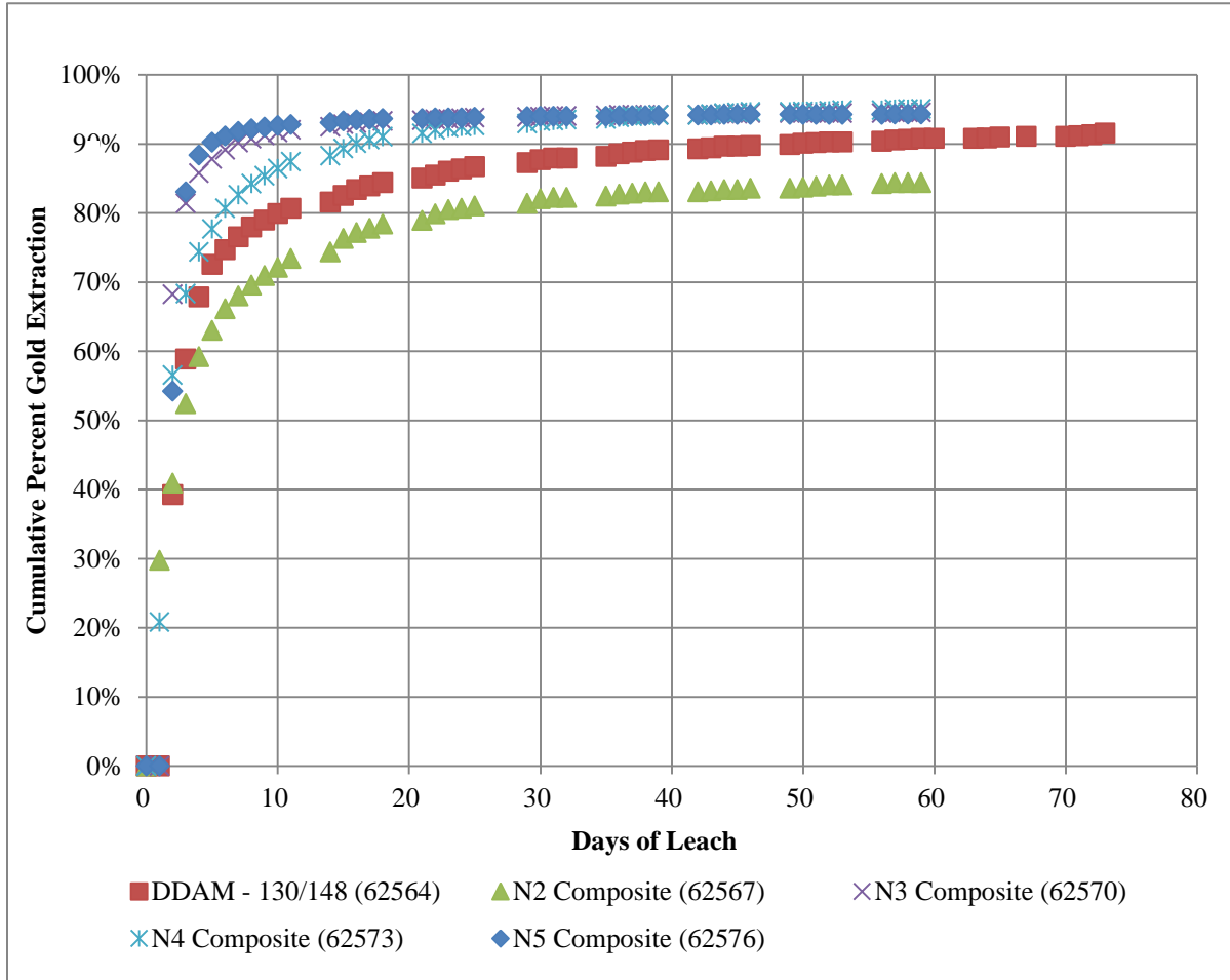
Figure 2: Gold Leach Curves
