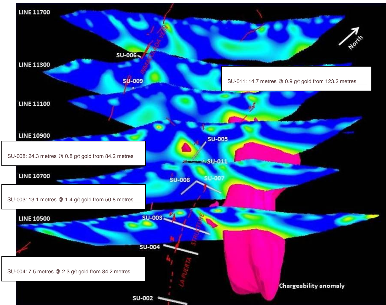
Figure 3. Three-dimensional model of the IP chargeability at La Puerta (magenta = high, blue = low)
