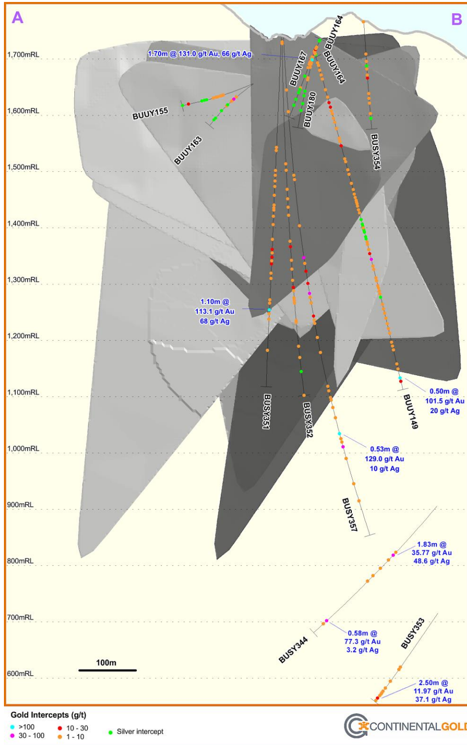
Figure 2 – Long Section, Veta Sur, showing new drilling highlights against the outlines of the October 2012 Veta Sur mineral resource envelope
