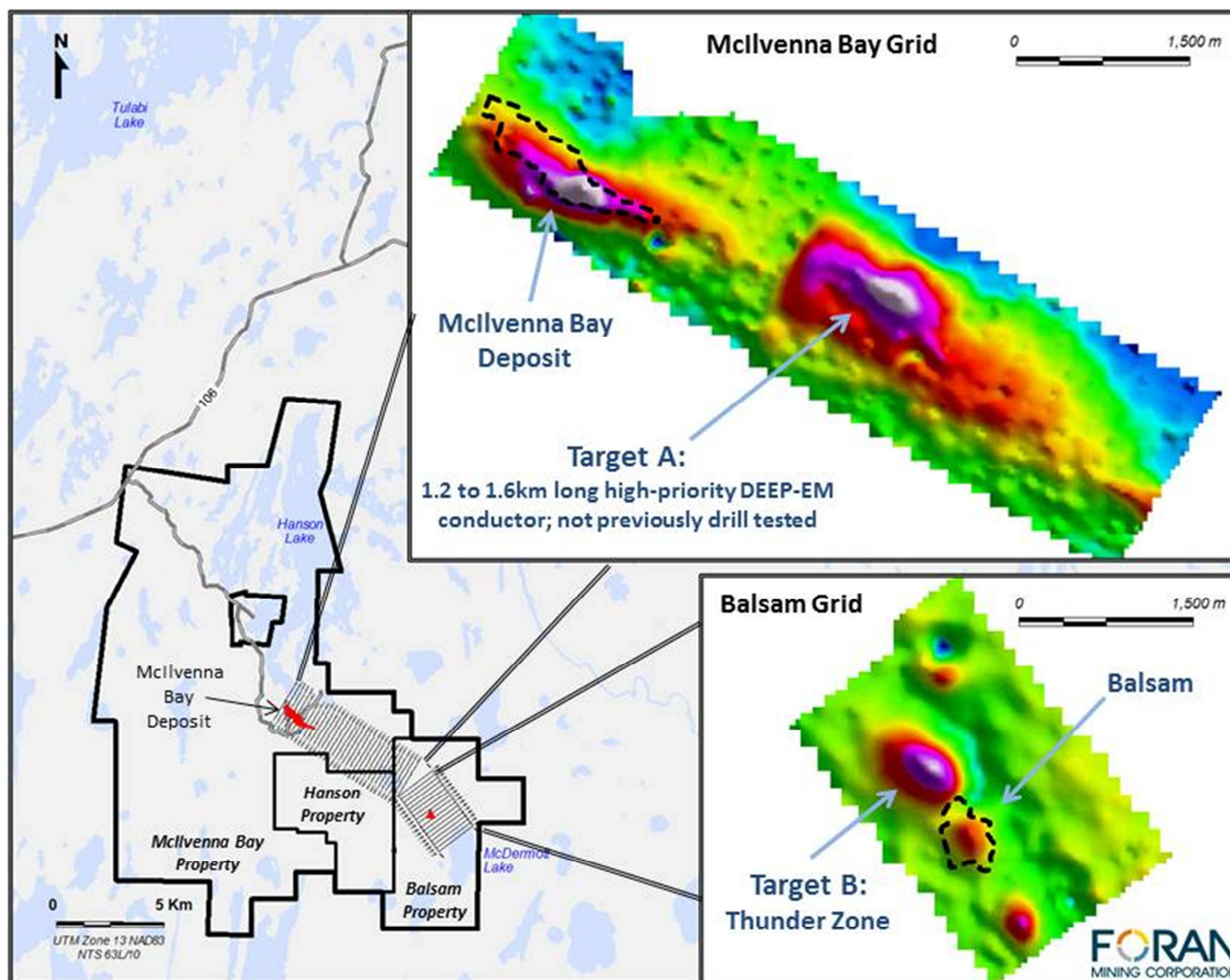
Figure 1. DEEP-EM survey location map for McIlvenna Bay and Balsam Grids. Inset of McIlvenna Bay is gridded mid- to late-time EM channel 20 – X component data using a linear and compressed colour scale. Inset of Balsam is gridded mid- to late-time EM channel 20-XYZ component data using a linear and compressed colour scale.
