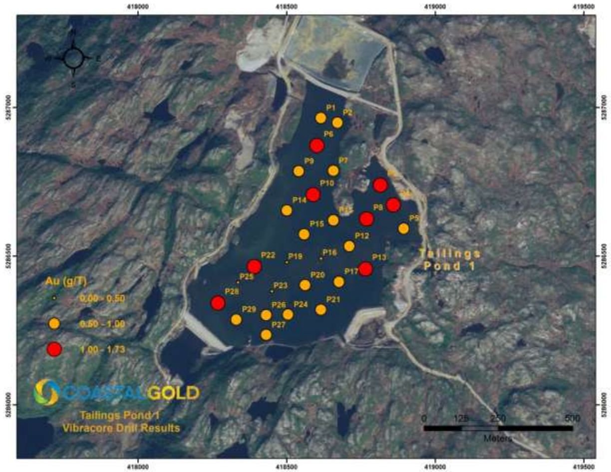
FIGURE 1: TAILINGS POND 1 DRILL HOLE RESULTS, HOPE BROOK GOLD PROJECT
