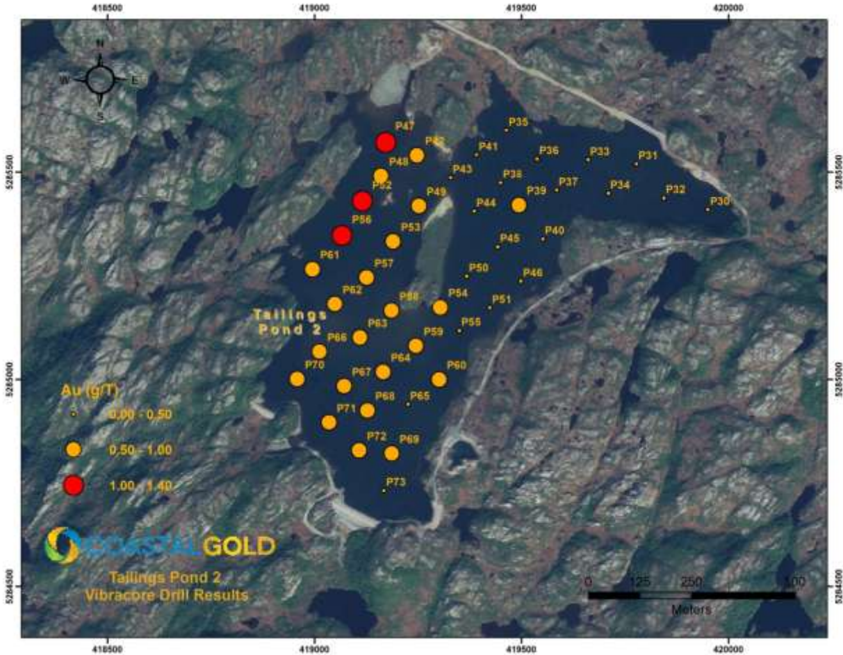
FIGURE 2: TAILINGS POND 2 DRILL HOLE RESULTS, HOPE BROOK GOLD PROJECT
