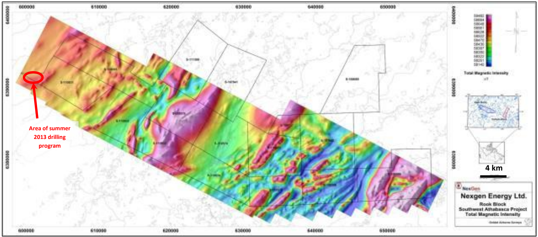
Fig 3 Rook area, TMI magnetics
