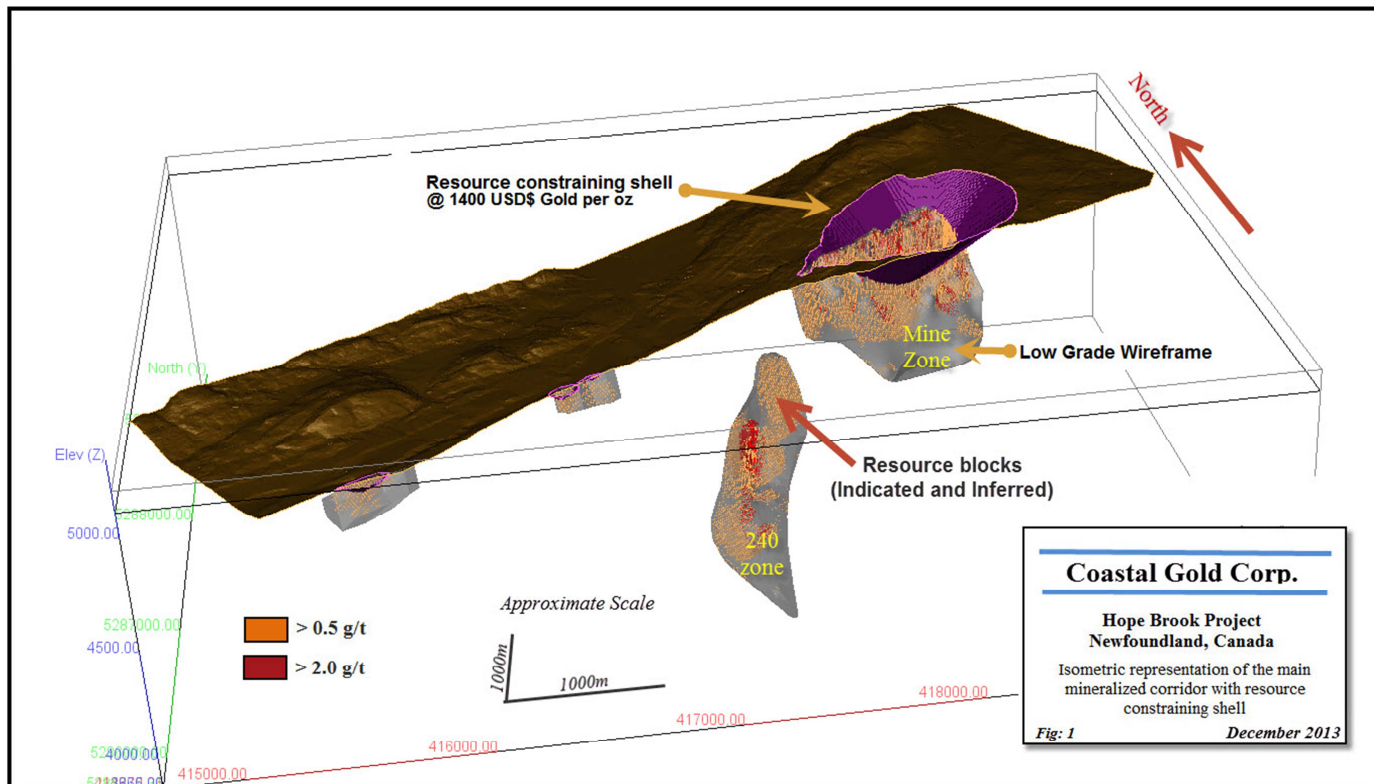
Figure 1: Isometric Representation of the Main Mineralized Corridor with Resource Constraining Shell
