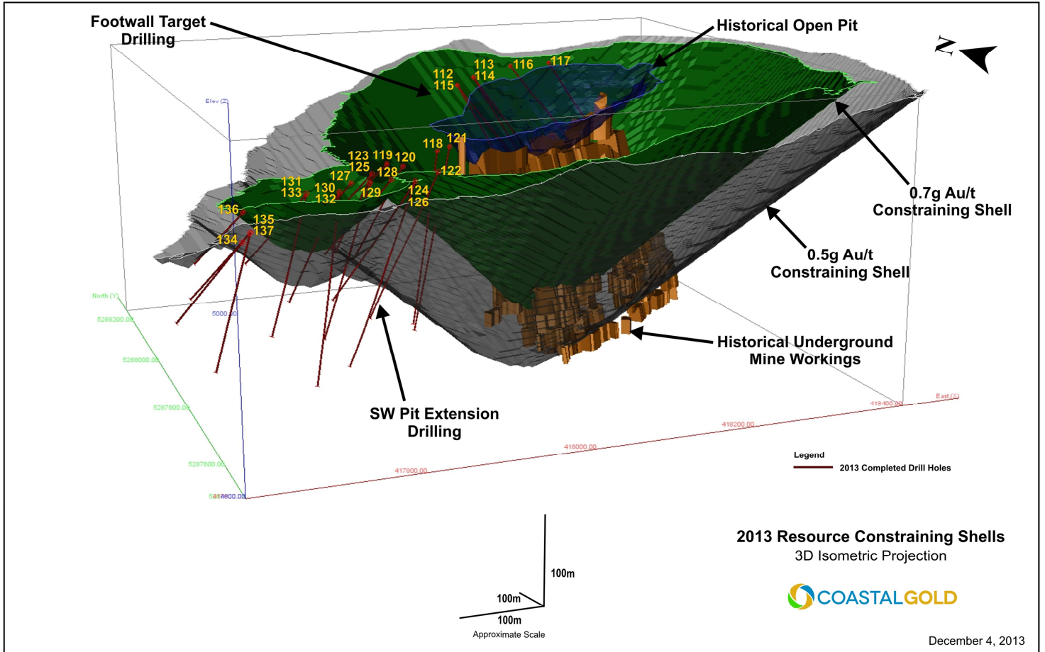
Figure 2: 3D Isometric Projection of 2013 Resource Constraining Shell
