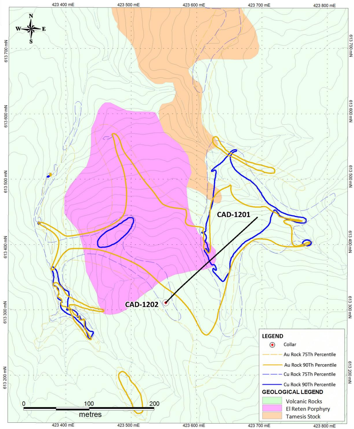
Figure 1: Surface geology at the El Retén target, showing the traces of the first two drill holes as well as the surface geochemical anomalies for gold and copper.
