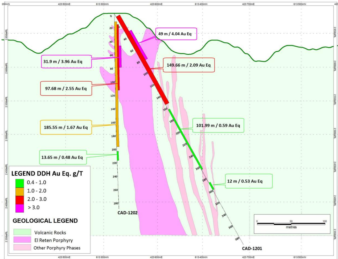
Figure 2: Cross-section showing drill holes CAD-1201 and CAD-1202 with the mineralized intervals included in Table 2 and interpreted geology.
