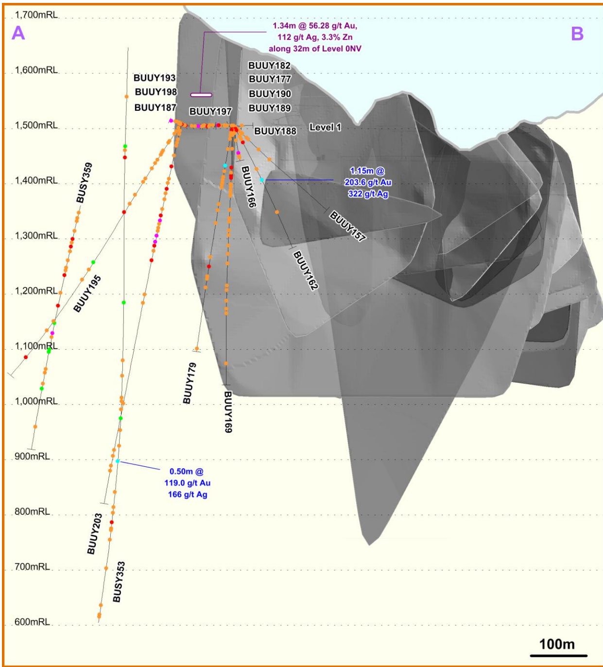
Figure 2 – Long Section, Yaraguá, showing highlights of new drilling and underground sampling results against the outlines of the October 2012 Yaraguá mineral resource envelope
