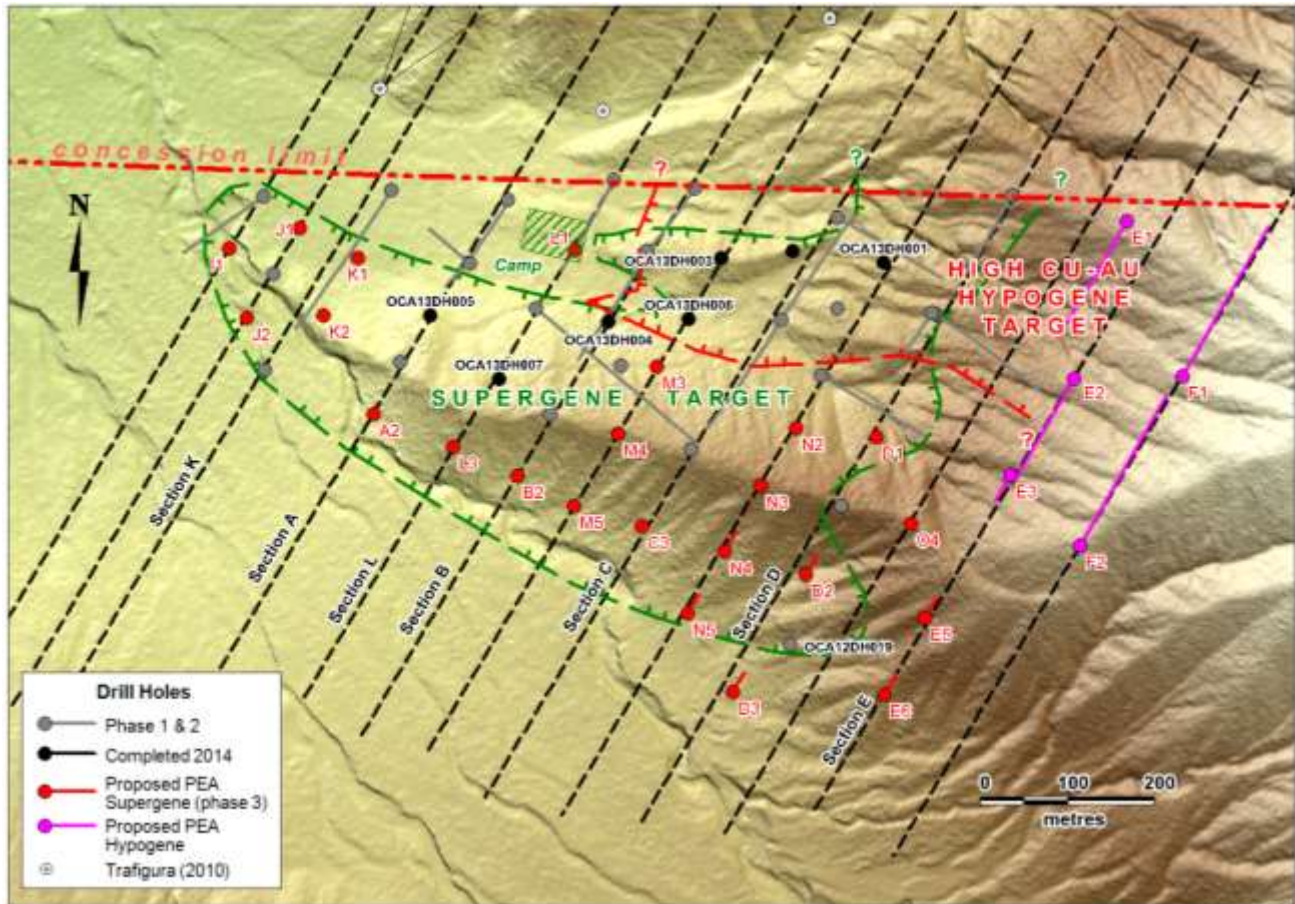
Figure 1: Map of proposed Phase 3 drill holes and local geology.
