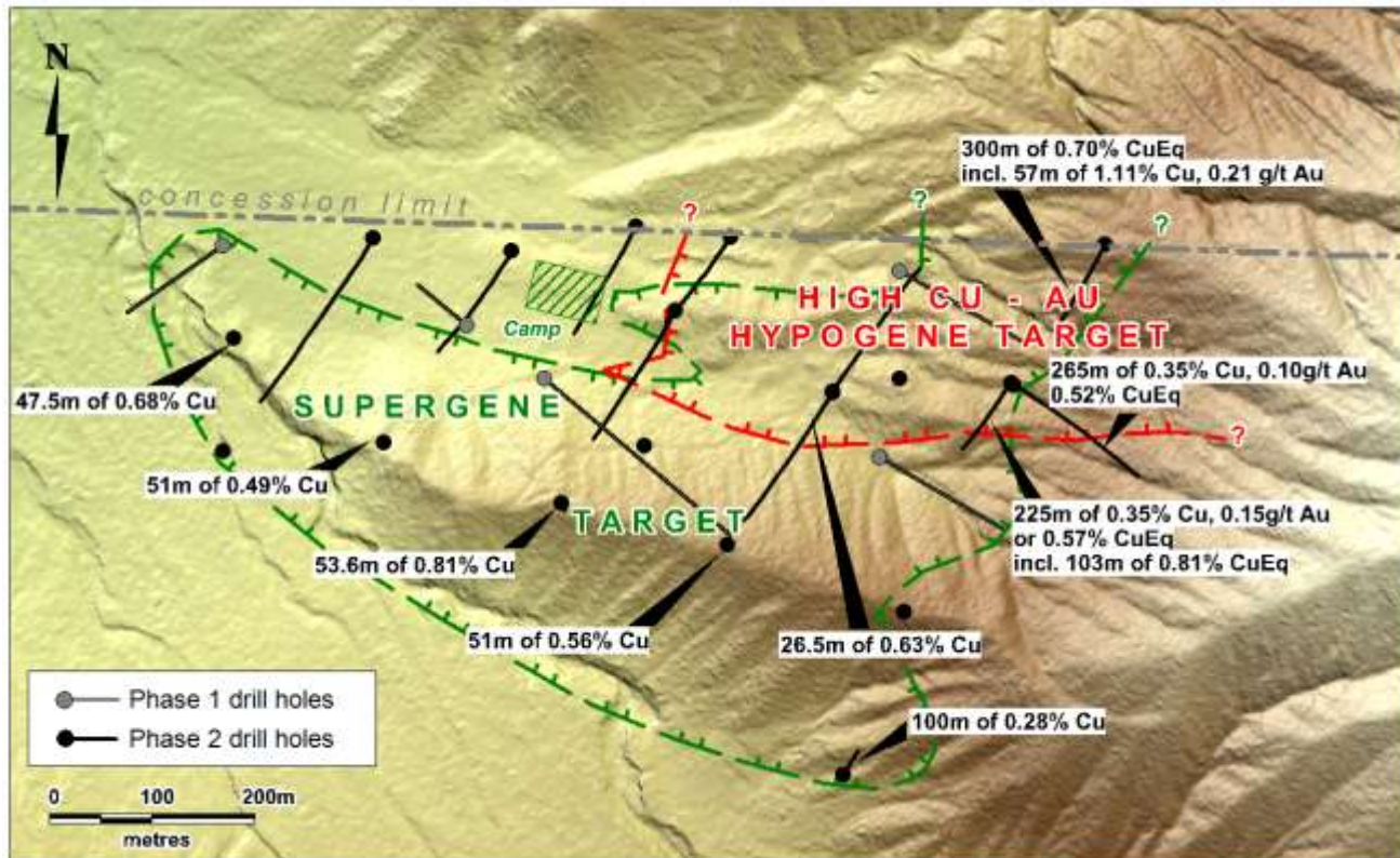
Figure 2: Map of Phase 2 programme highlights.
