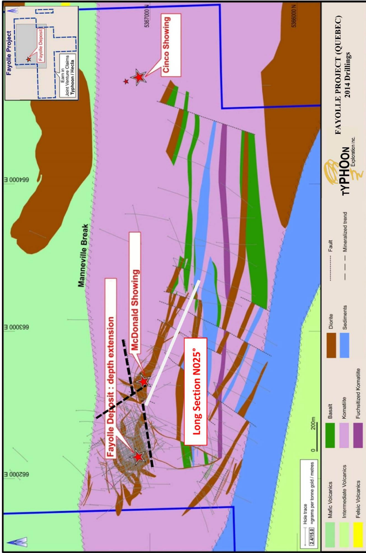
Figure 1 : Fayolle Property geology and targets locations
