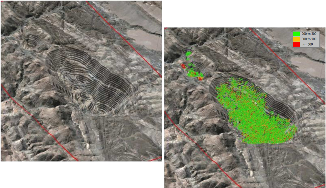
Figure 2. Valencia pit design (left) with the higher grade resource blocks within the pit (right). Mining licence boundary shown in red. (view NE)
