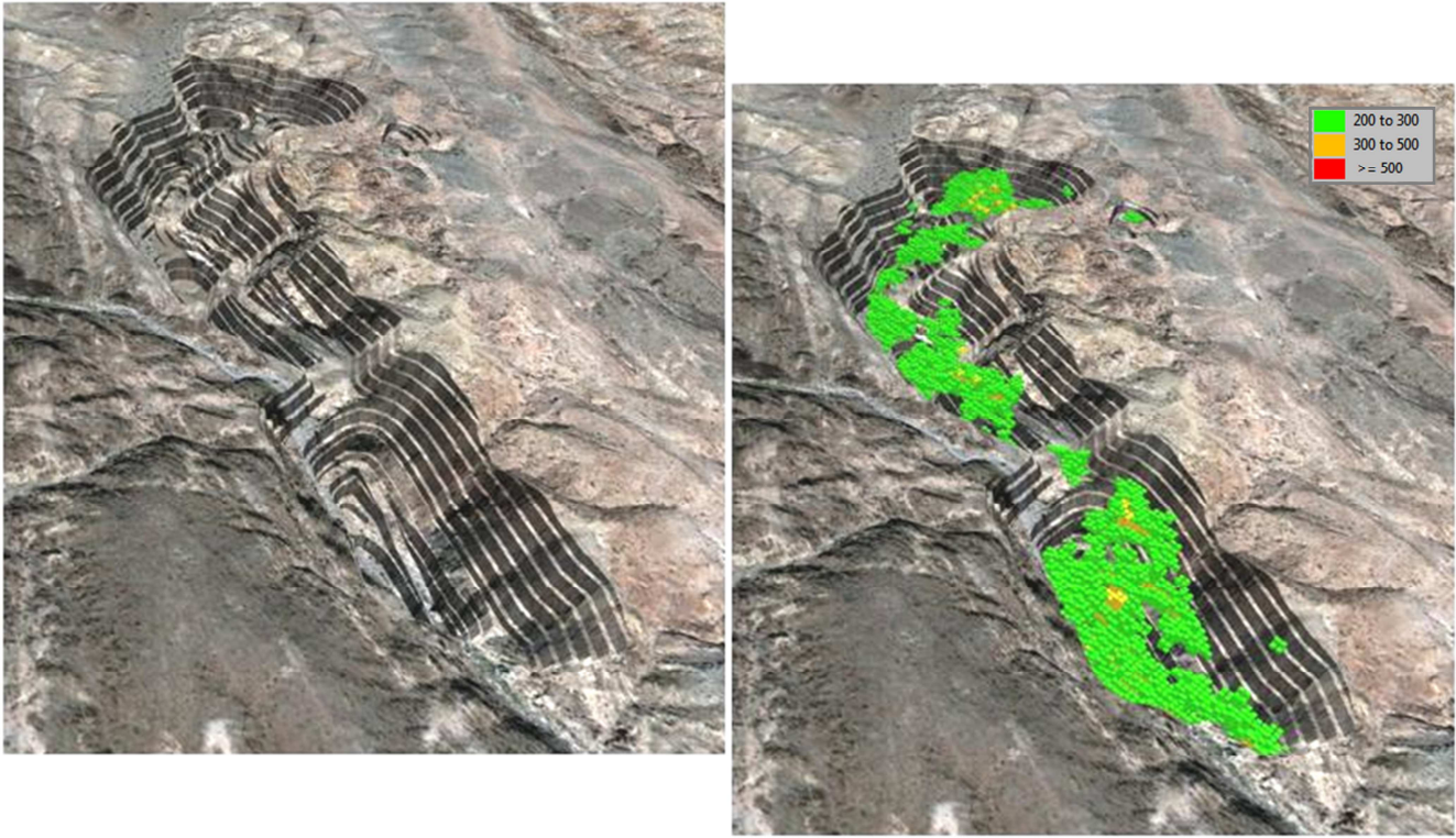
Figure 3. Namibplaas pit design (left) with the higher grade resource blocks within the pit (right). (view SW)
