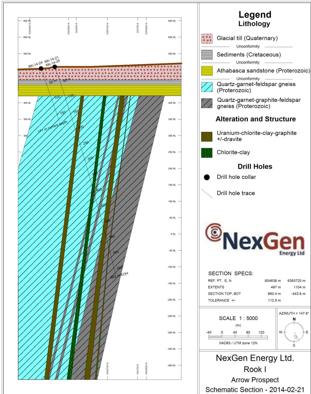
Figure 2 Schematic Section of RK-14-21
