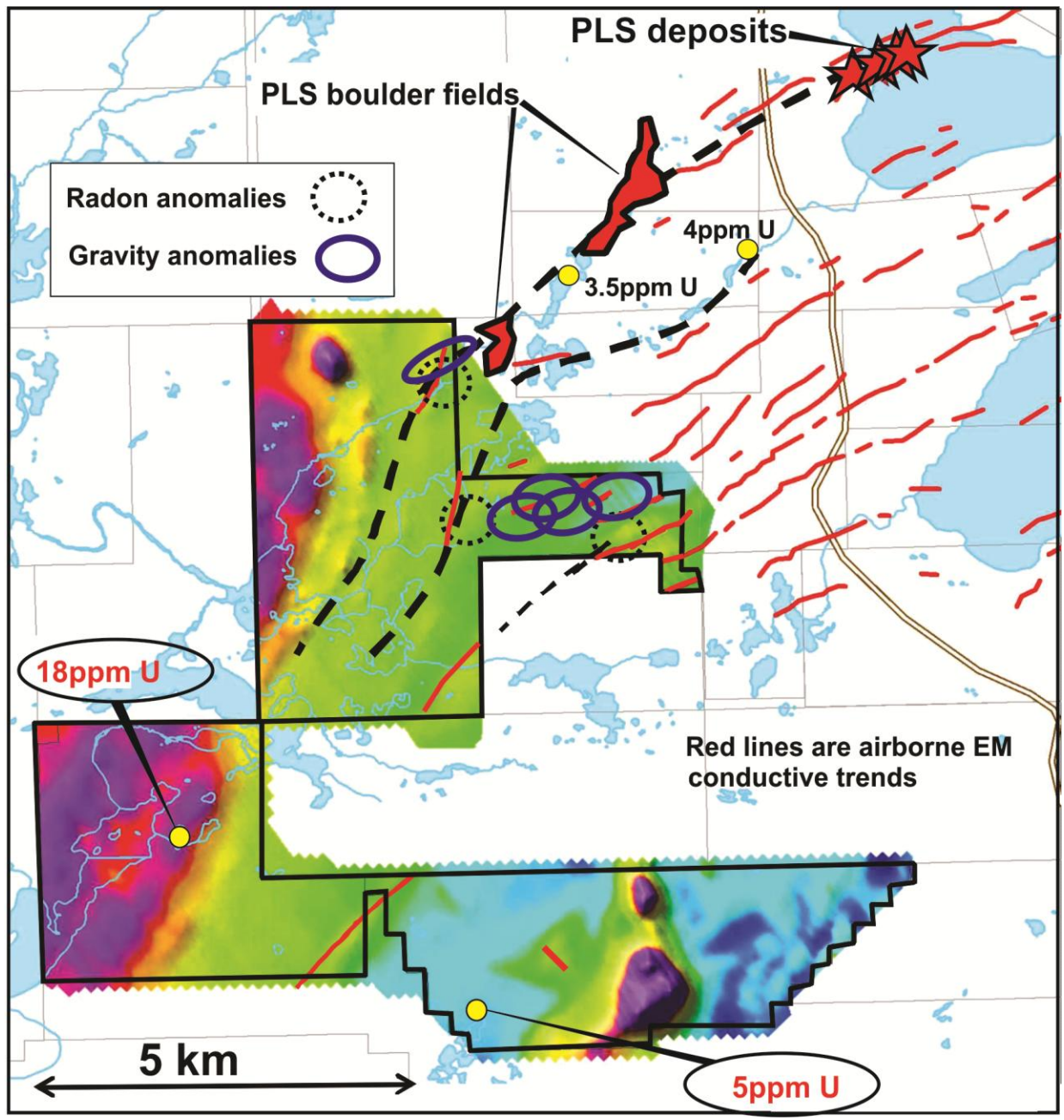
Figure 1: Gravity and radon anomalies with EM conductors on Forum's Clearwater Project. Red lines are airborne EM conductors, black dashed lines are interpreted structural trends. Yellow circles are locations of anomalous lake sediment samples. The background colours are from an airborne magnetometer survey.
