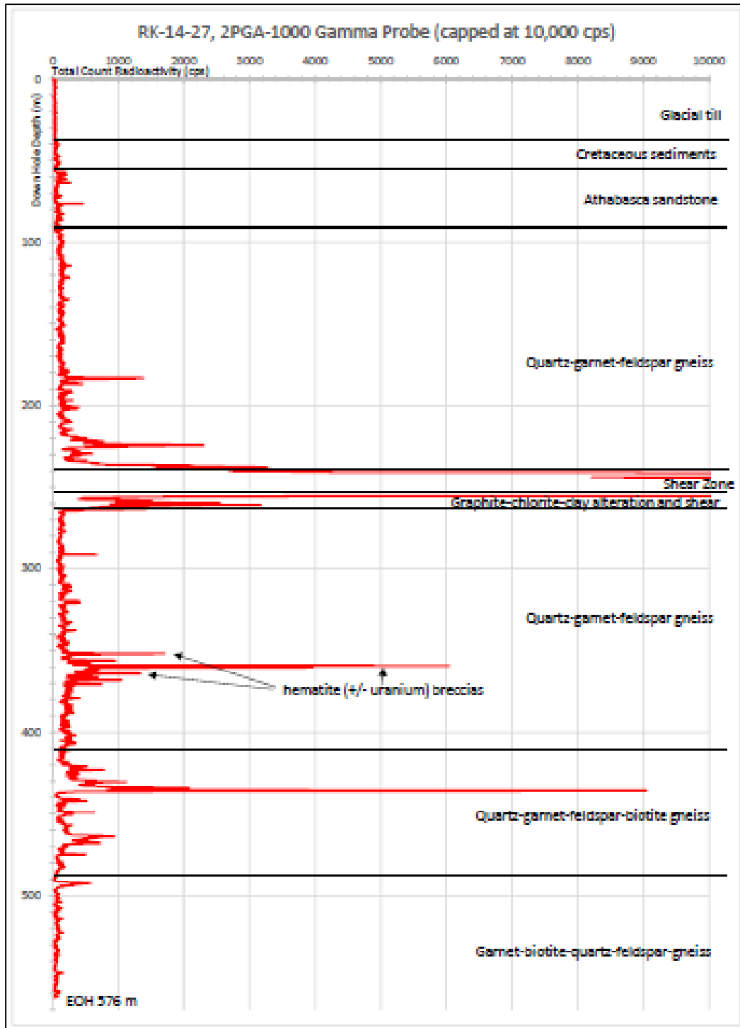
Fig 4 Arrow, RK-14-27, 2PGA-1000 downhole probe results (capped)
