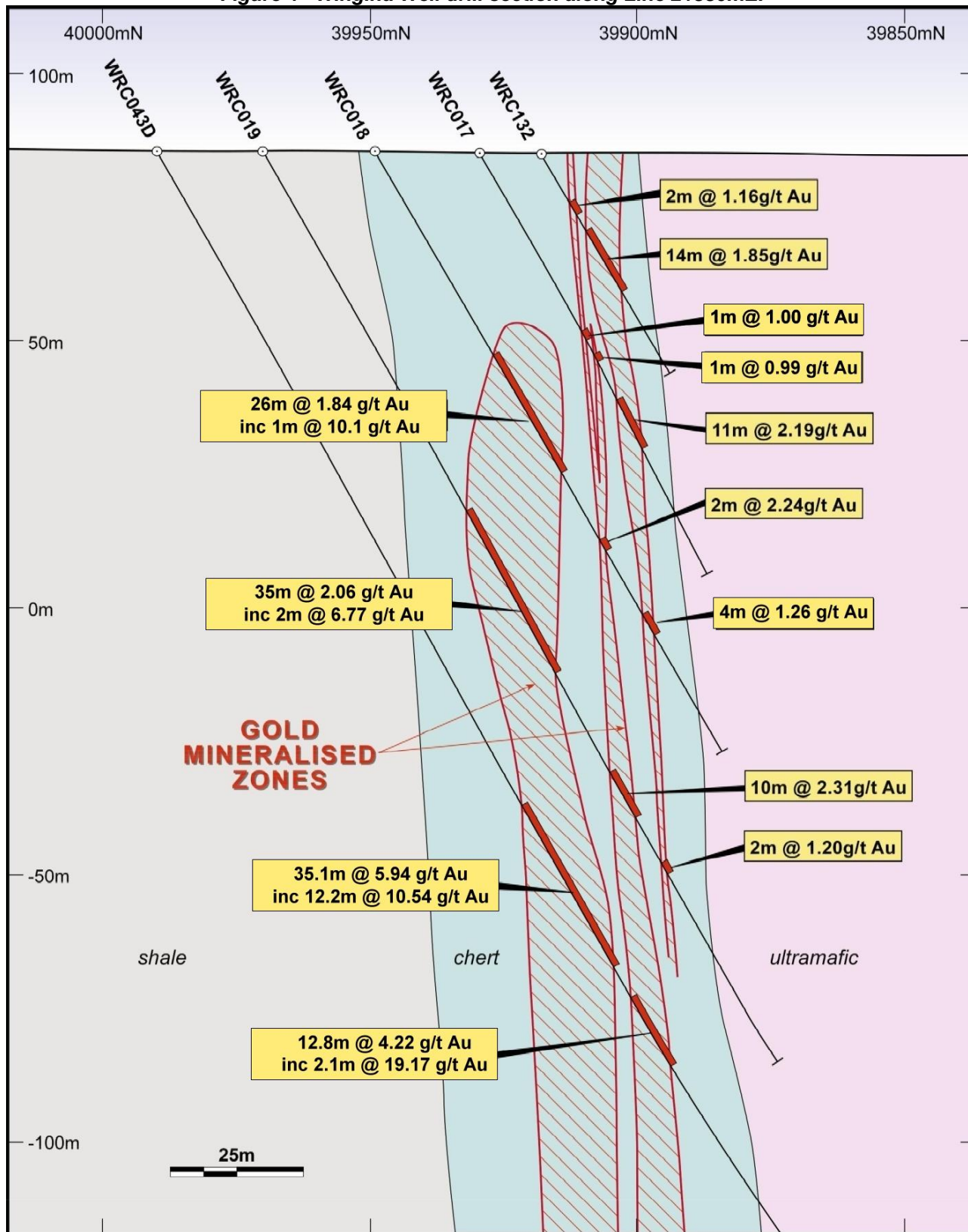
Figure 4– Wingina Well drill section along Line 21880mE.
