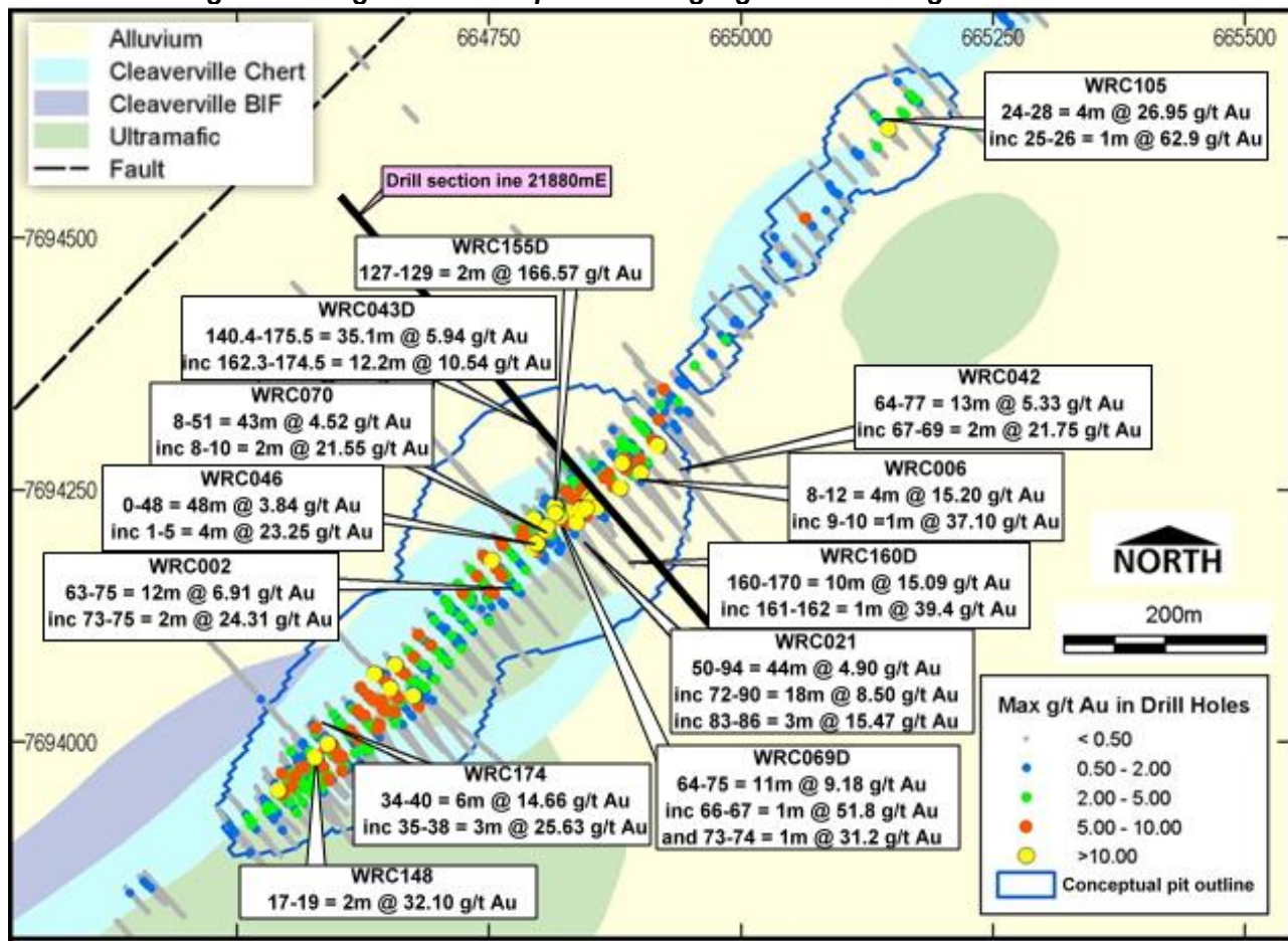
Figure 3: Wingina Well drill plan showing significant drilling intersections.
