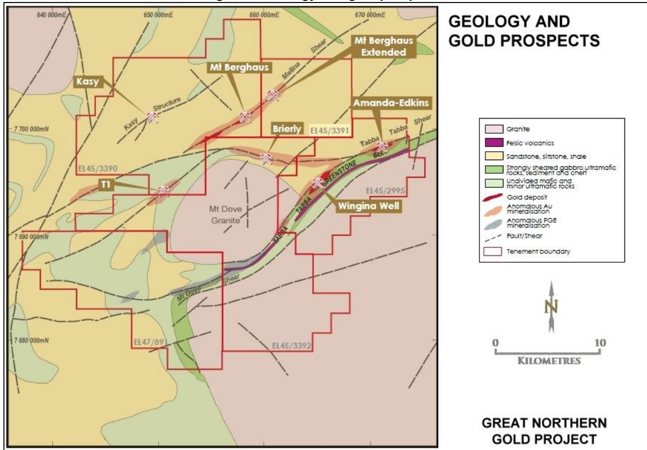
Figure 2: Geology and gold prospects
