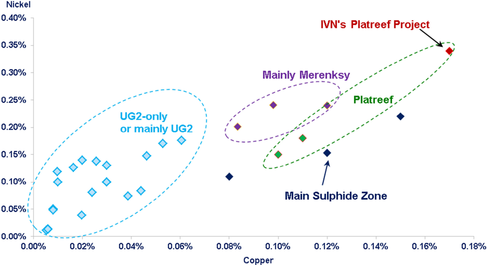
Figure 2: Base-metal (nickel and copper) concentrations by PGM-bearing reef.
