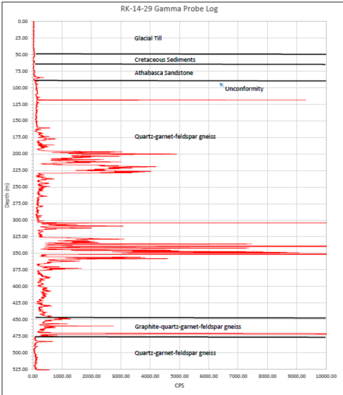
Fig 3 Arrow, RK-14-29, 2PGA-1000 downhole probe results (capped)
