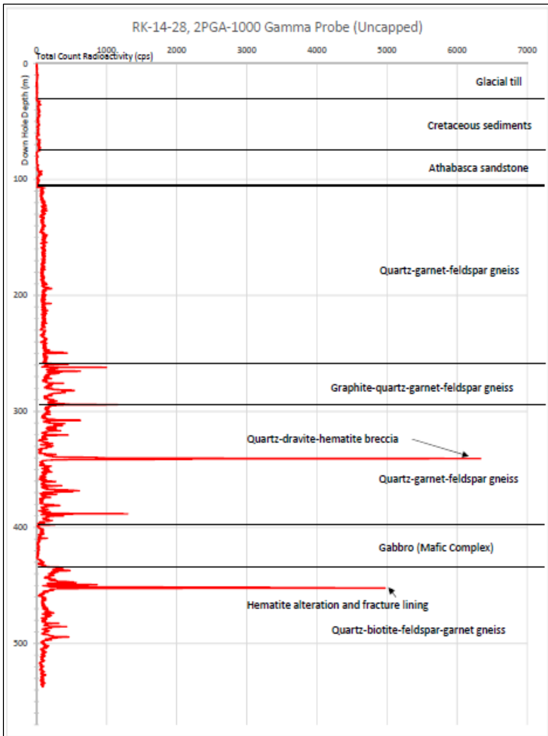
Fig 4 Arrow, RK-14-28 (gravity target), 2PGA-1000 downhole probe results (uncapped)
