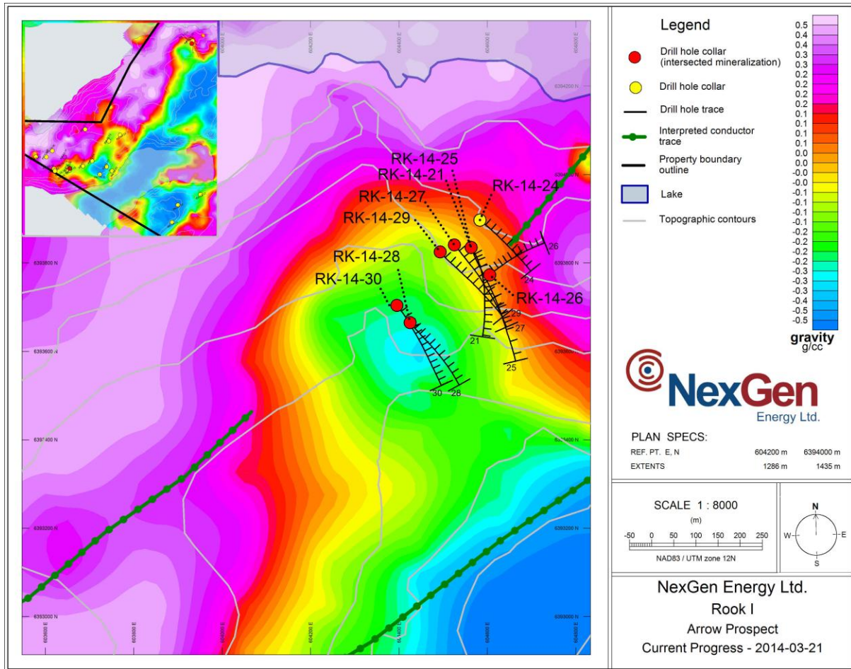
Fig 1 Arrow, drill hole locations (gravity background)
