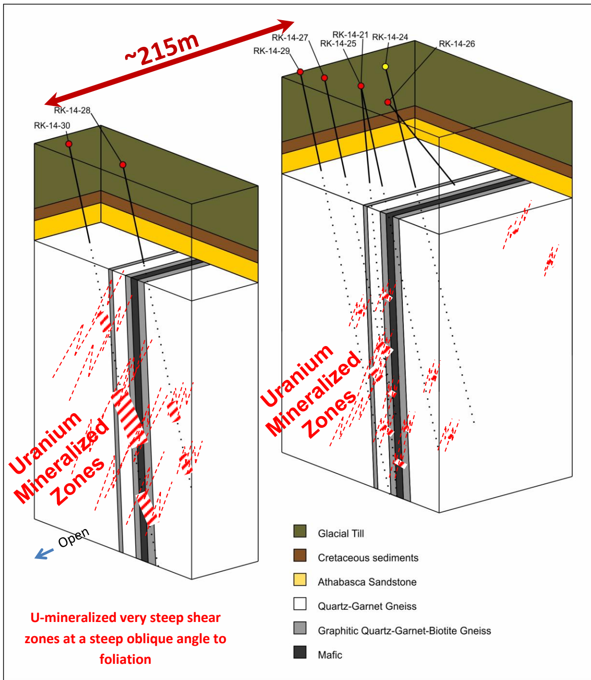
Fig 7 Arrow: schematic 3D representation of the Arrow mineralized system
