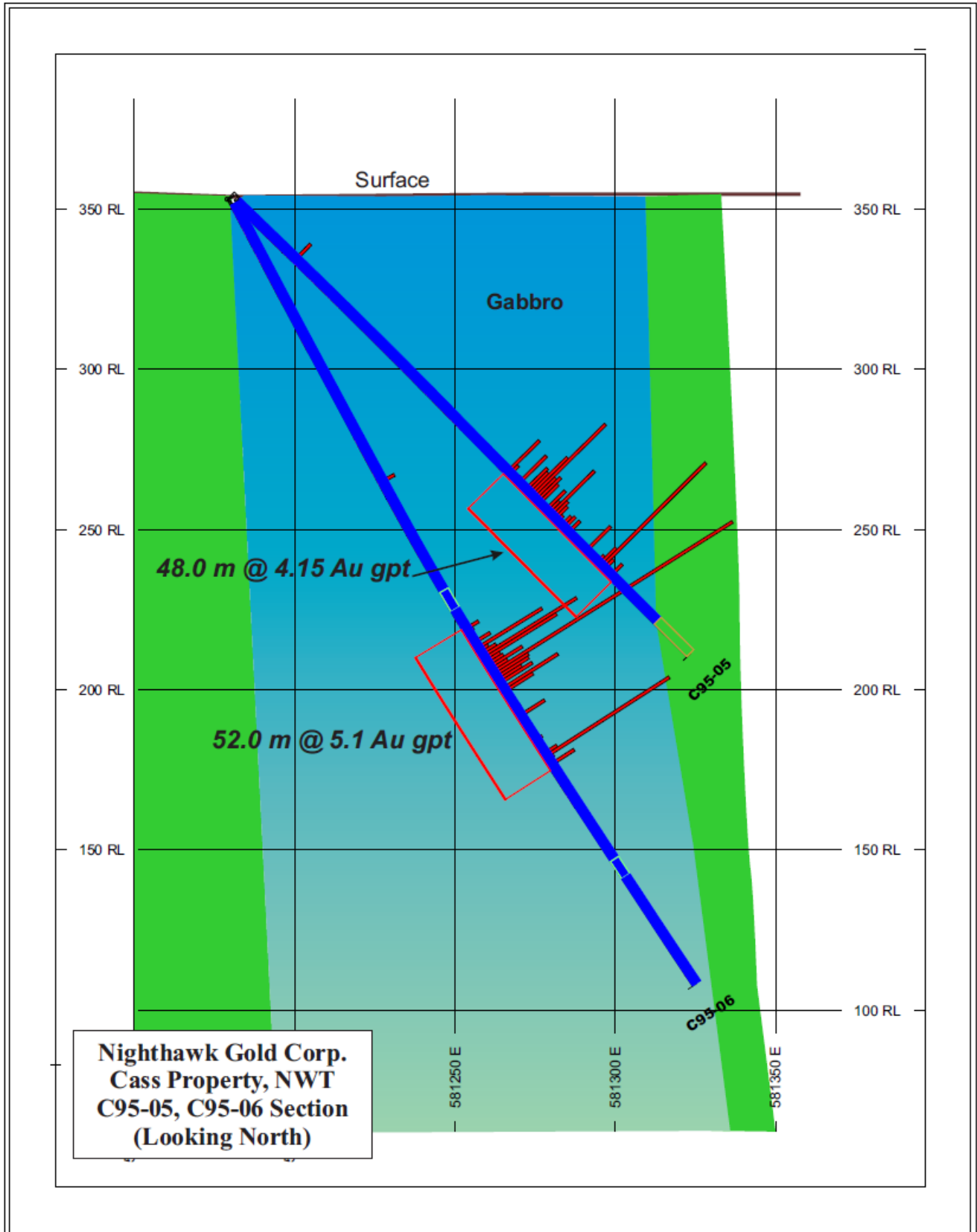
Figure 2. – Cross Section of Holes C95-05 and C95-06 at Cass
