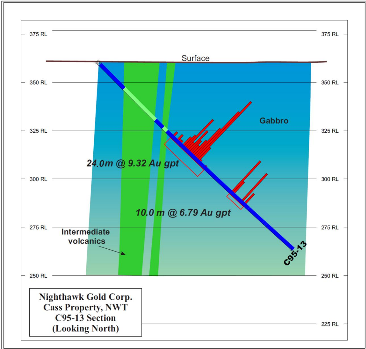
Figure 3. – Cross Section of Hole C95-13 at Cass
