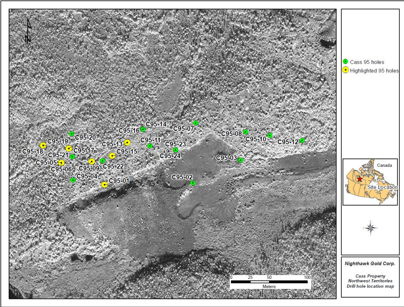
Figure 1. – 1995 Drill Hole Location Map at Cass
