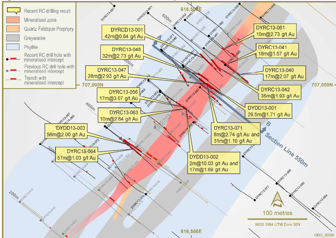
Figure 2 – Drill Hole Locations and Selected Intercepts
