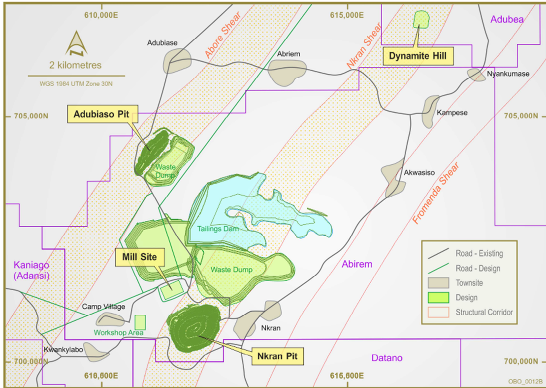
Figure 1 Dynamite Hill Location Map and Proposed Phase 1 Infrastructure for the Asanko Gold Mine
