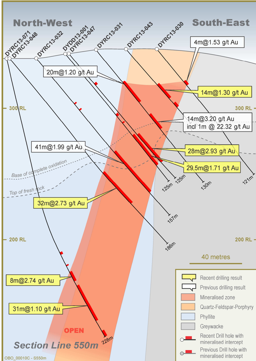
Figure 3 – Section Line 550m with Select Drill Intercepts
