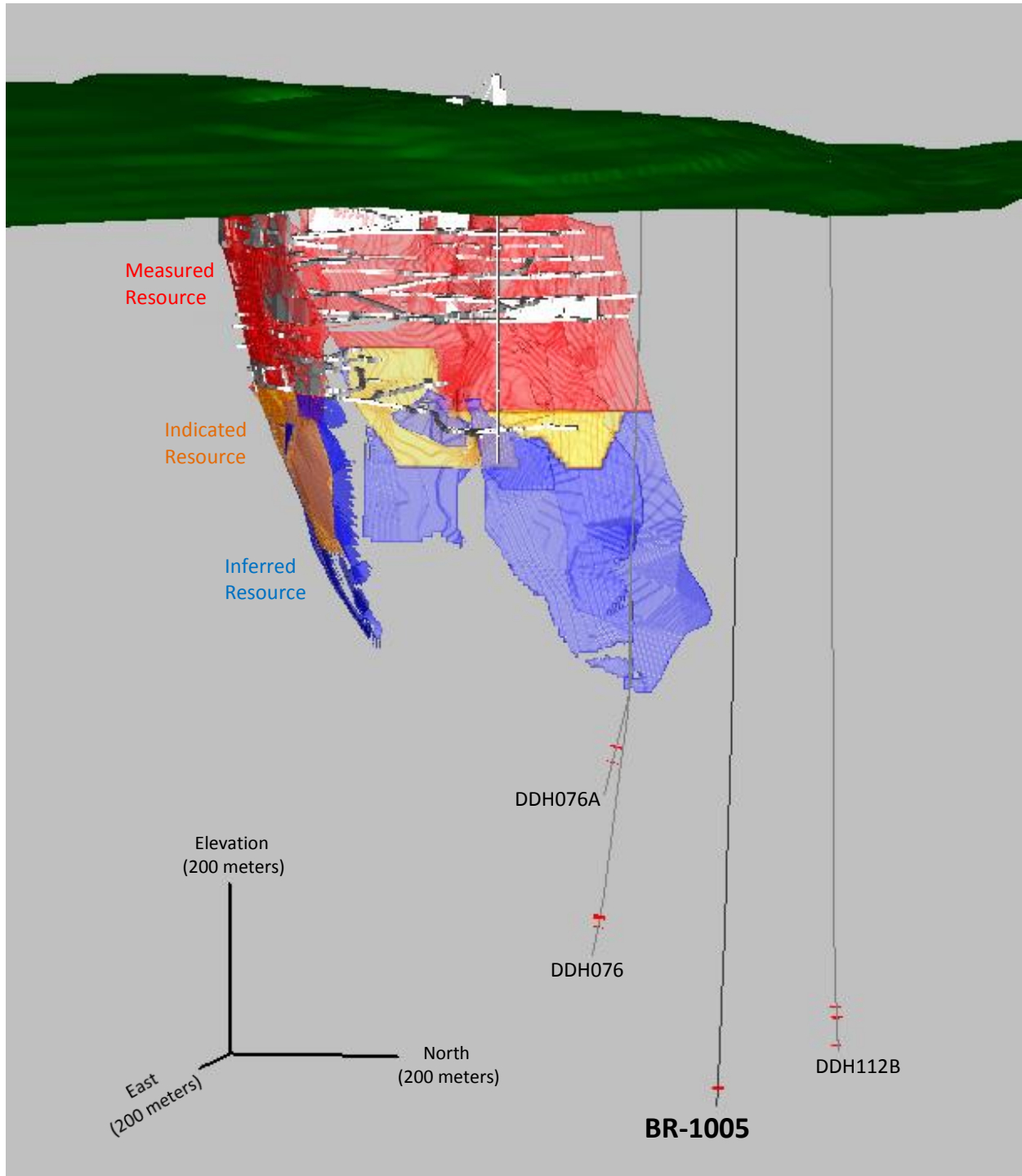
Figure 1: 3D View (Looking N260° -5°) of the Caribou deposit and drill hole BR-1005
