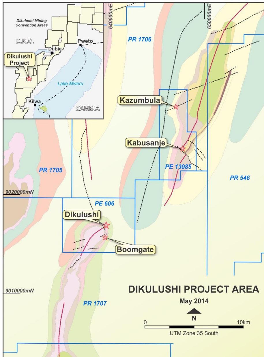
Figure 1: Copper deposits in Dikulushi District
