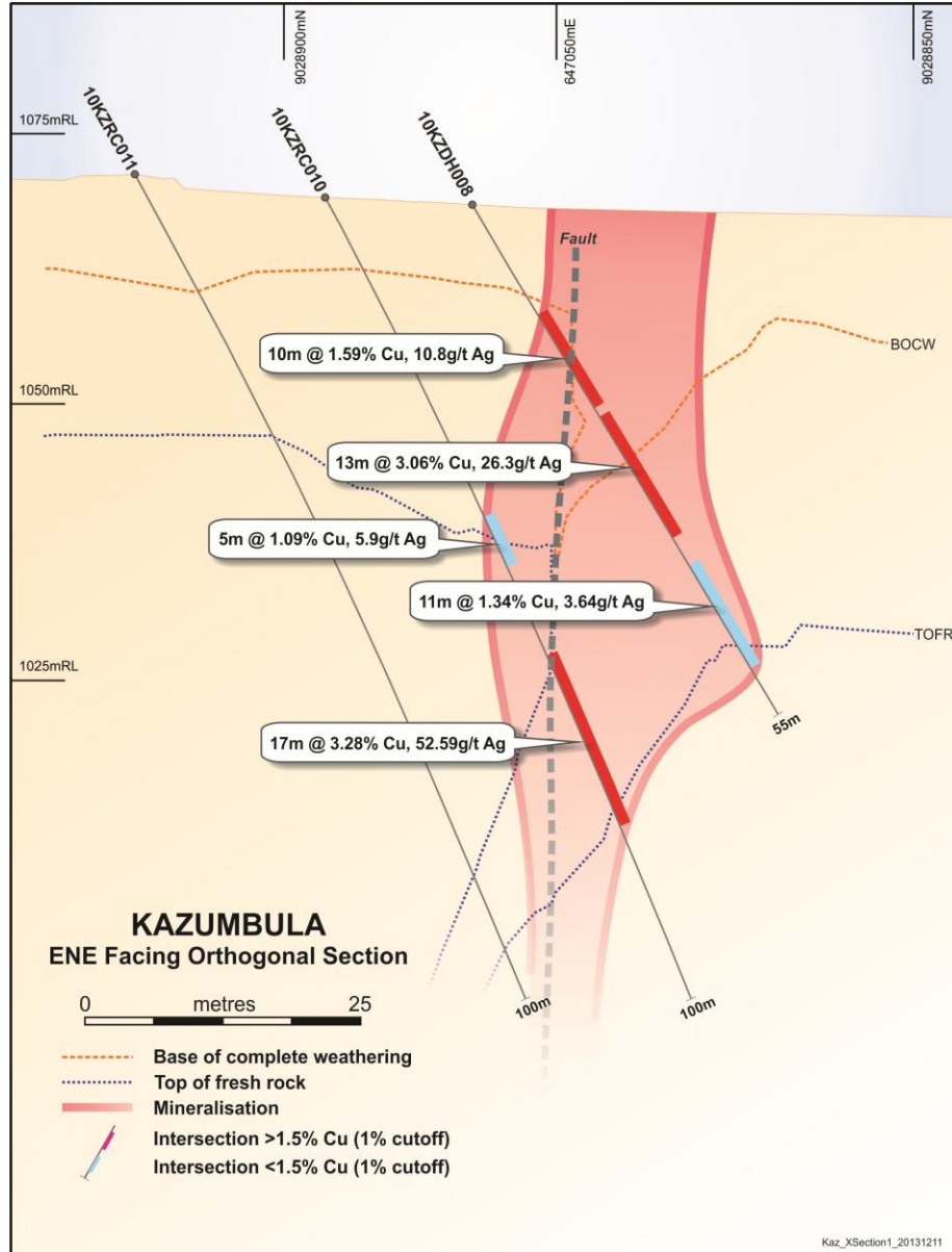
Figure 2: Drill cross-section through Kazumbula deposit
