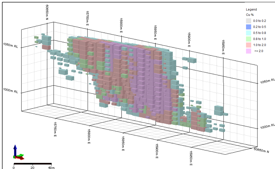
Figure 3: Kazumbula Mineral Resource model perspective view looking NW
