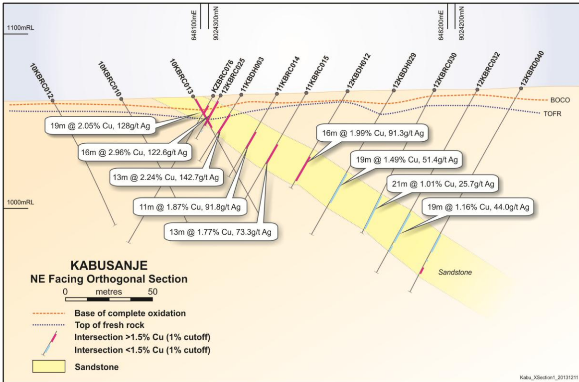
Figure 4: Drill cross-section through Kabusanje deposit
