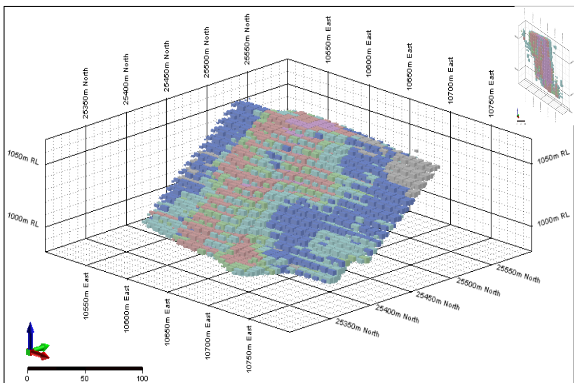
Figure 5: Kabusanje Mineral Resource model perspective view looking NE.
