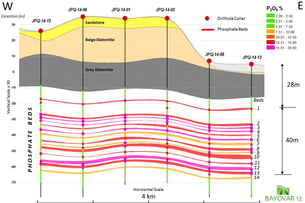
Section 1 Interpretive Geological Section : Holes JPQ -14-15, 06, 01, 03, 18, 13
