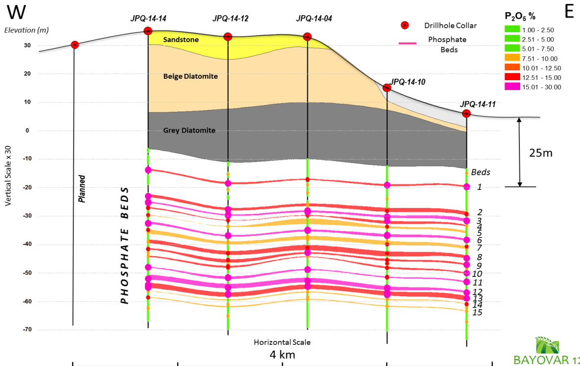
Section 2 Interpretive Geological Section : Holes JPQ -14-14, 12, 04, 10, 11
