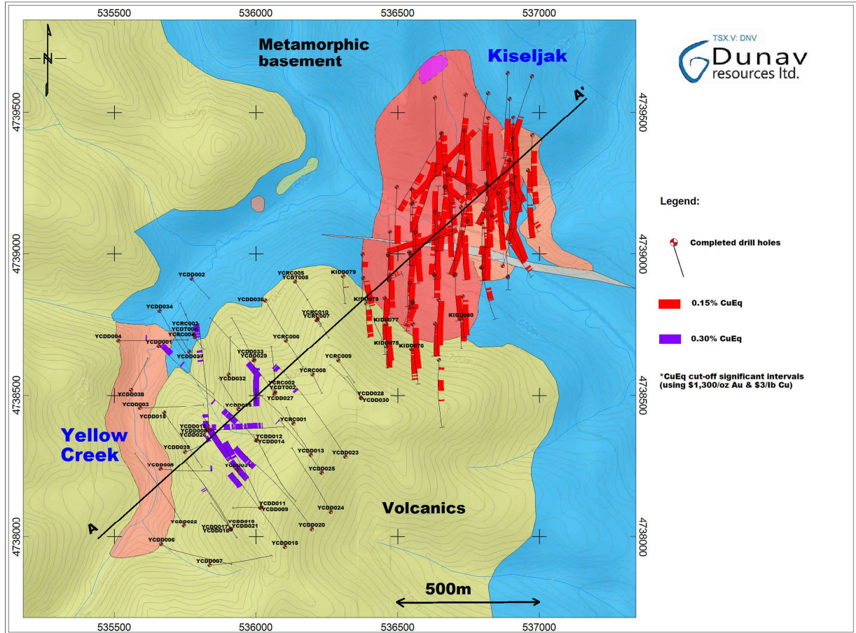
Figure 1: Plan view of the Kiseljak and Yellow Creek areas showing Dunav drilling to date (section line A-A' relates to Figure 2). Note that the grid spacing is 500 meters.
