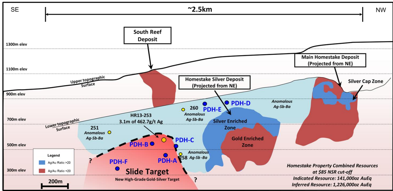
Figure 1: Longitudinal section showing approximate targeting for the first six proposed drill holes on the Slide target at the Homestake Ridge property.
