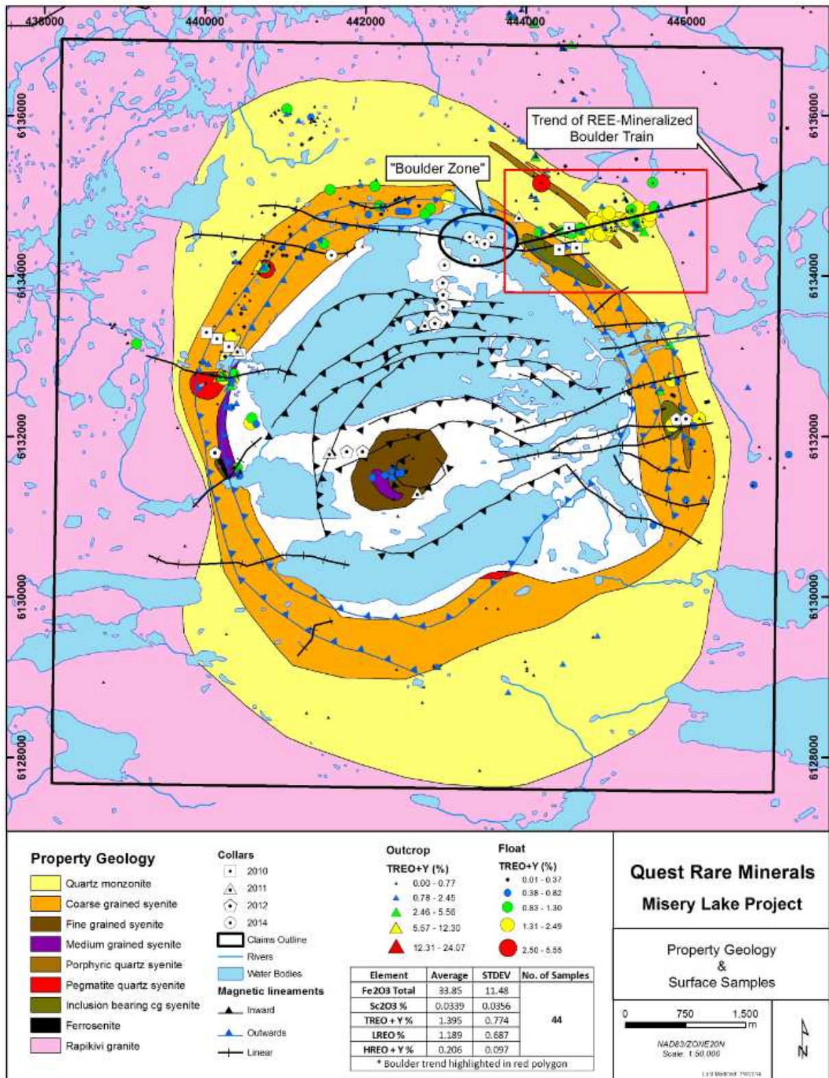
Figure 3 – Property Geology Map, Misery Lake Project, Québec
