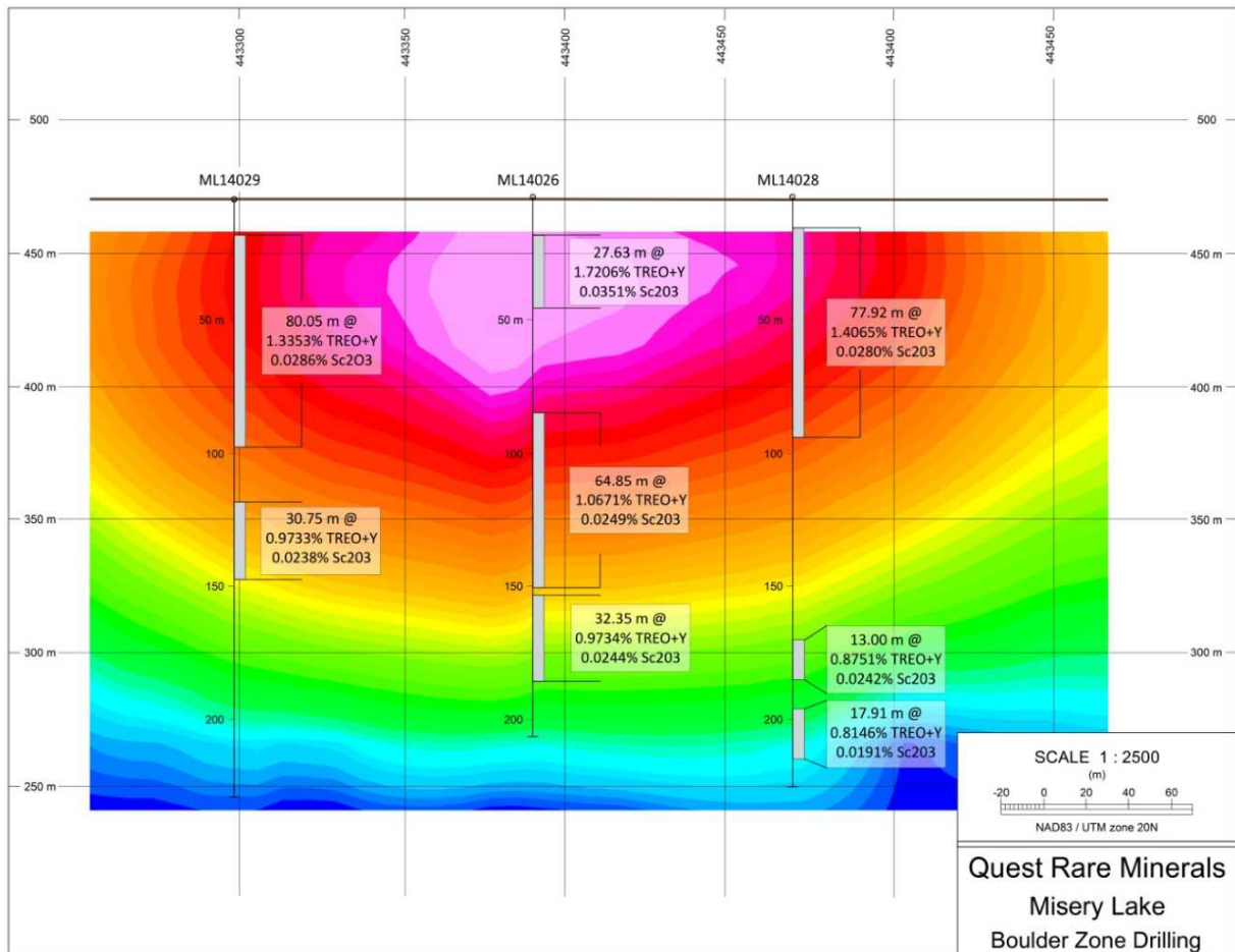
Figure 4 – Drilling Cross-section with Intersection Assays on a Magnetics Base, Misery Lake Project, Québec
