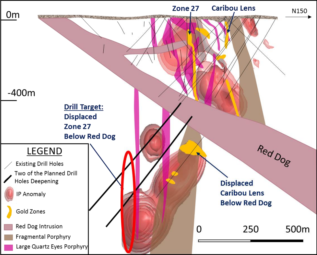
Figure 2 – Vertical Cross-section 2525 E. Deepening two of the existing drill holes to test the displaced Zone 27 below the Red Dog intrusion.
