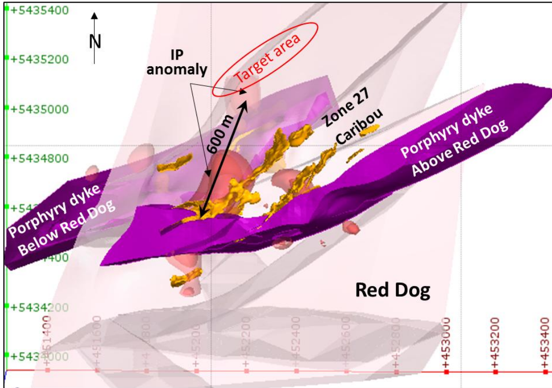
Figure 1 – New target area below the Red Dog intrusion. Plan view (from 0 to -800 meters). Geology and mineralization below Red Dog is displaced by as much as 600 meters to the NNE.
