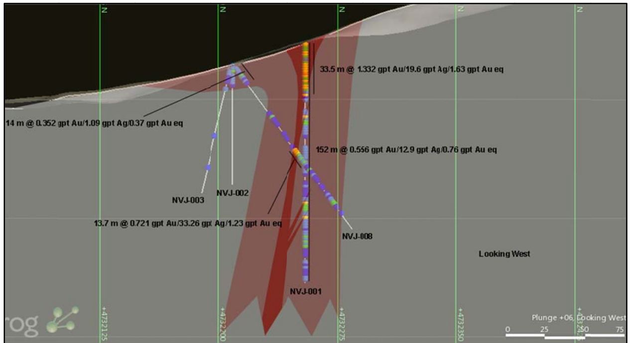
Figure 4 – Cross Section through NVJ-001, 002, & 003 and NVJ-008 (Western-most Section)
