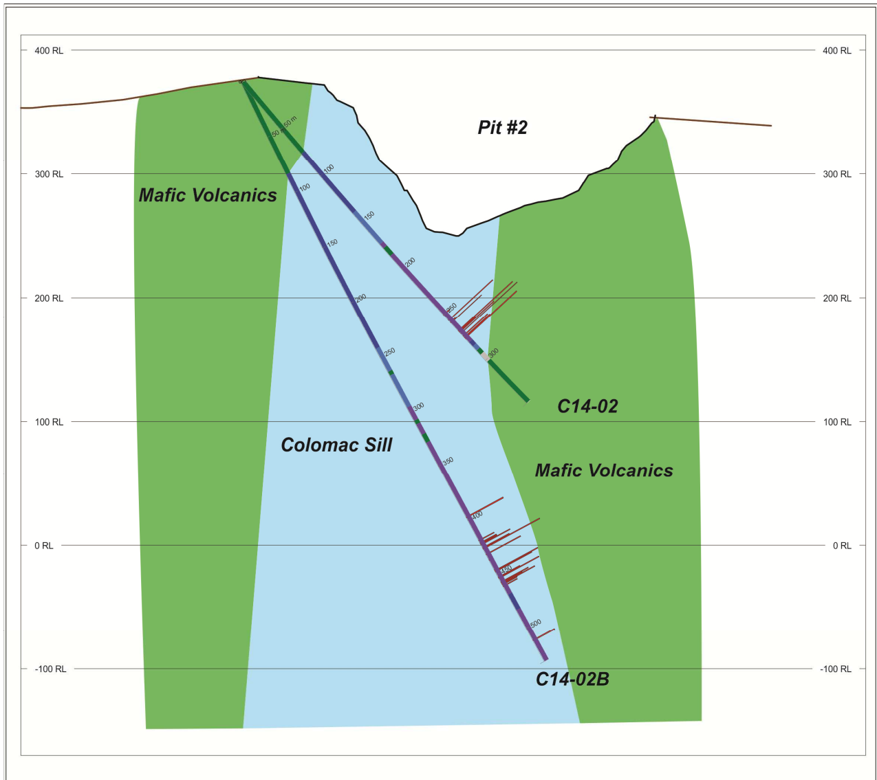
Figure 5. Cross Section – Colomac Holes C14-02 and C14-02B
