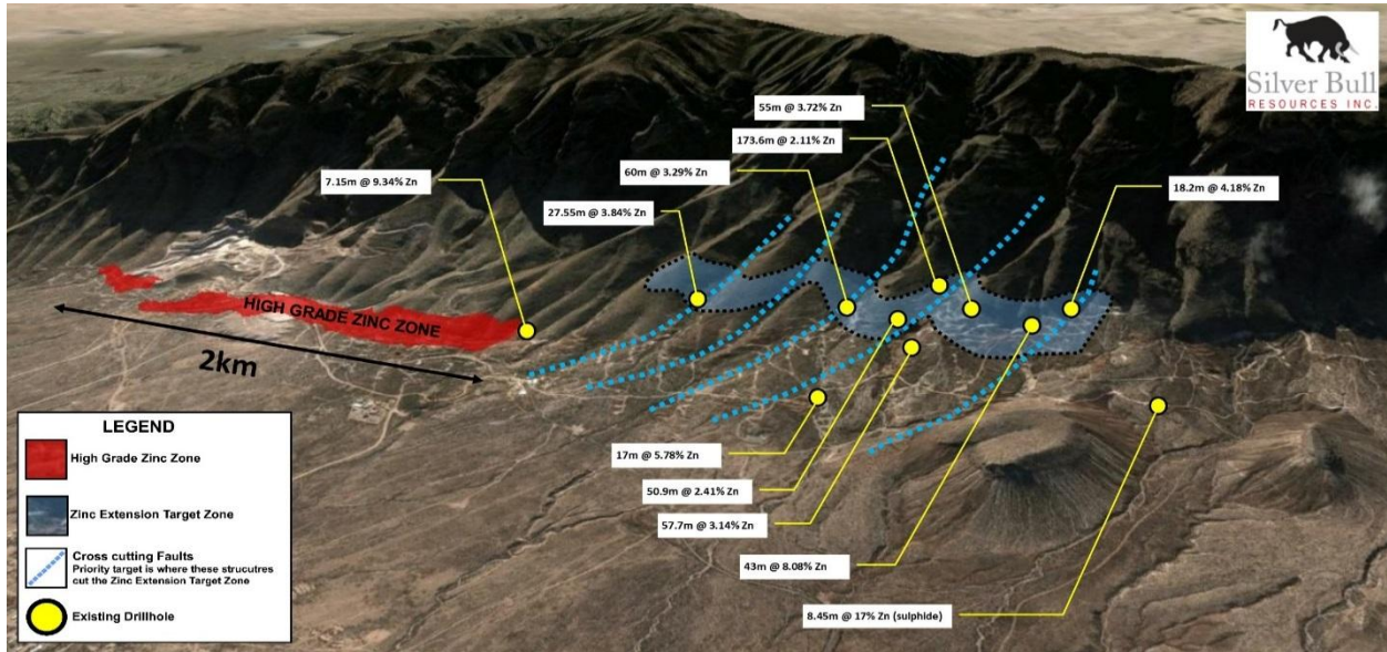
Figure 1. Target Zone of exploration upside (blue) relative to the existing High Grade Zinc Zone. Highlight holes from drilling targeting the silver mineralization are also shown and suggest a possible extension to the high grade zinc. Zones where N-S trending structures cut the "Zinc Extension target zone" will be the priority drill targets for any future exploration drilling.
