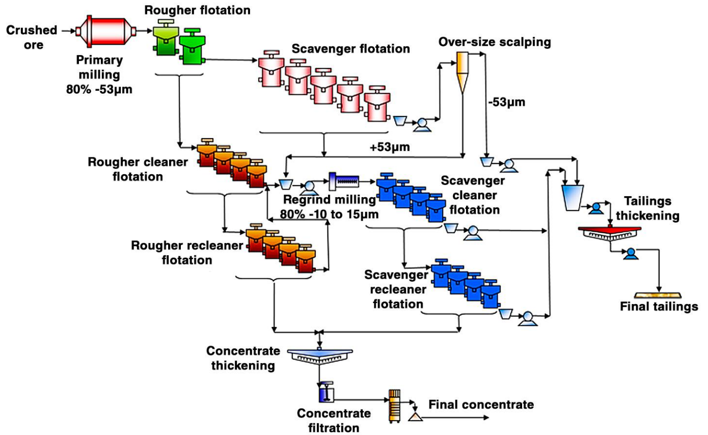
Figure 1: Laboratory flowsheet.
